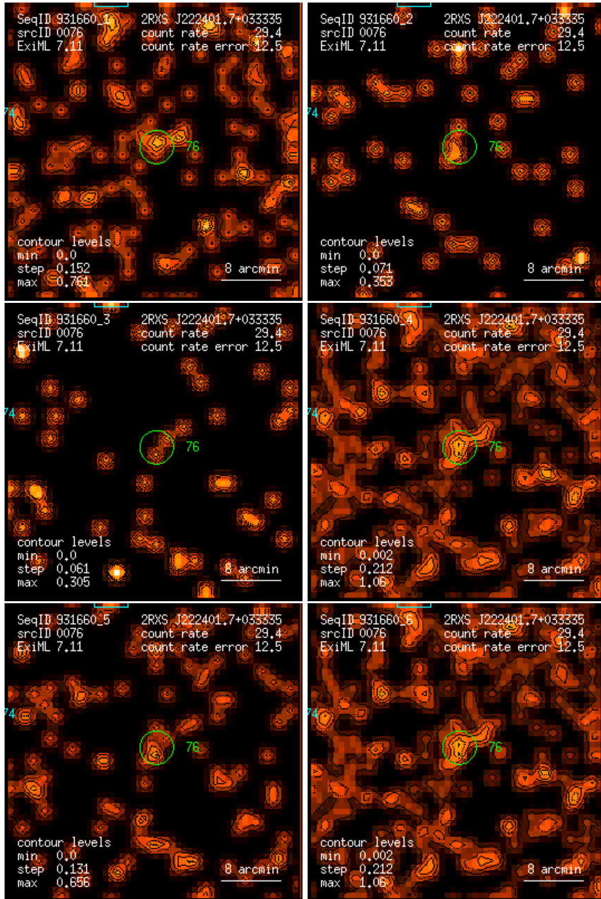
Figure 76: RASS 931660: detection 0076: band rate images, Gaussian filter: (1) PSPC channels 11 – 41, (2) 52 – 90, (3) 91 – 201, (4) 11 – 235, (5) 52 – 201, (6) 11 – 201. Broad band rates in counts/ks. Band rate contour levels in counts/ks/arcmin 2 .
