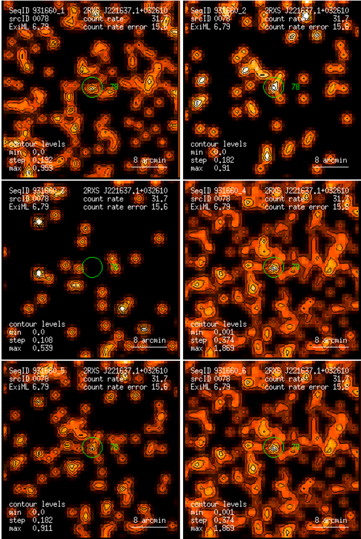
Figure 78: RASS 931660: detection 0078: band rate images, Gaussian filter: (1) PSPC channels 11 – 41, (2) 52 – 90, (3) 91 – 201, (4) 11 – 235, (5) 52 – 201, (6) 11 – 201. Broad band rates in counts/ks. Band rate contour levels in counts/ks/arcmin 2 .
