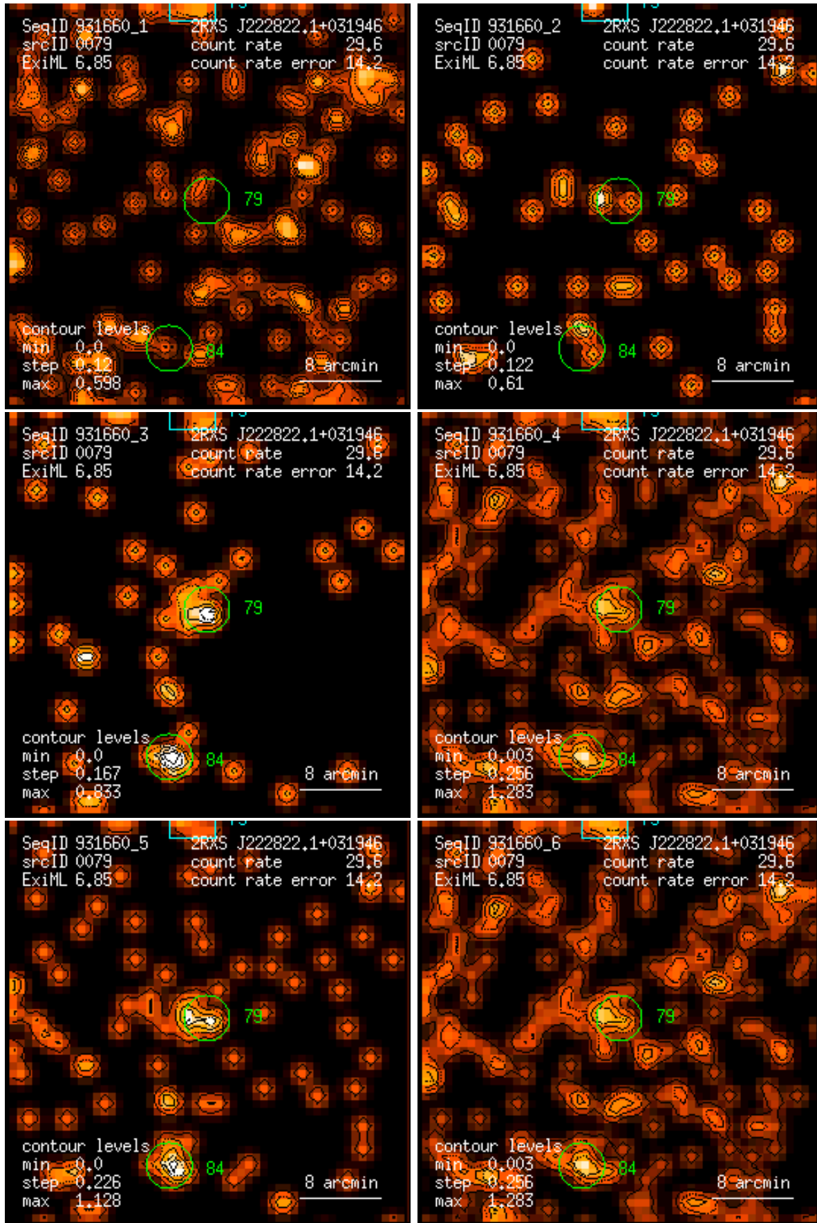
Figure 79: RASS 931660: detection 0079: band rate images, Gaussian filter: (1) PSPC channels 11 – 41, (2) 52 – 90, (3) 91 – 201, (4) 11 – 235, (5) 52 – 201, (6) 11 – 201. Broad band rates in counts/ks. Band rate contour levels in counts/ks/arcmin 2 .
