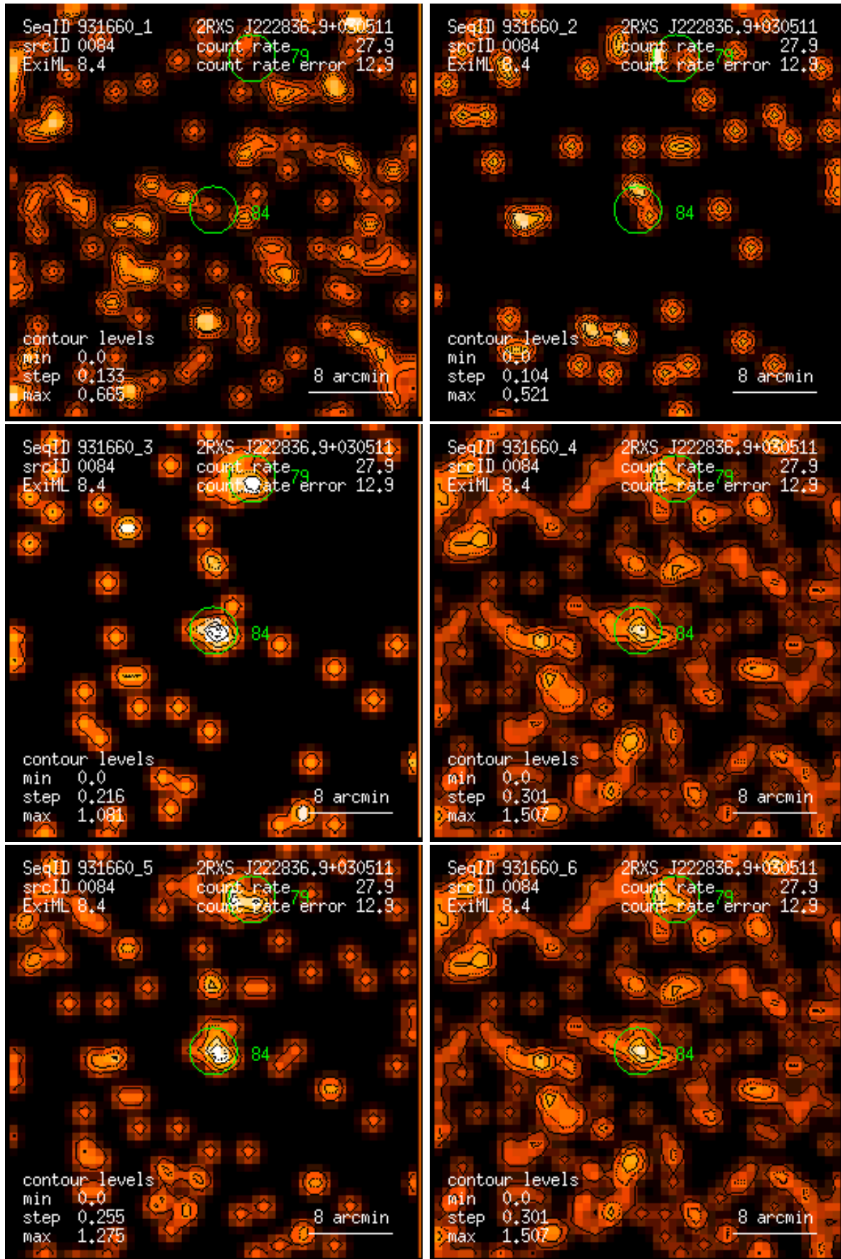
Figure 84: RASS 931660: detection 0084: band rate images, Gaussian filter: (1) PSPC channels 11 – 41, (2) 52 – 90, (3) 91 – 201, (4) 11 – 235, (5) 52 – 201, (6) 11 – 201. Broad band rates in counts/ks. Band rate contour levels in counts/ks/arcmin 2 .
