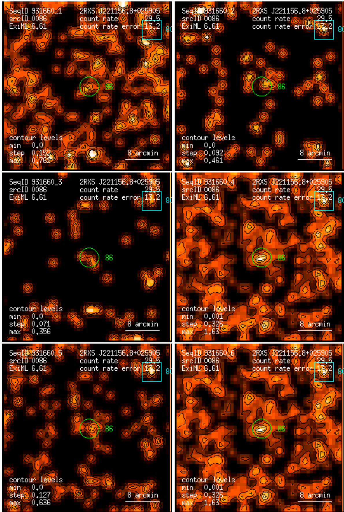
Figure 86: RASS 931660: detection 0086: band rate images, Gaussian filter: (1) PSPC channels 11 – 41, (2) 52 – 90, (3) 91 – 201, (4) 11 – 235, (5) 52 – 201, (6) 11 – 201. Broad band rates in counts/ks. Band rate contour levels in counts/ks/arcmin 2 .
