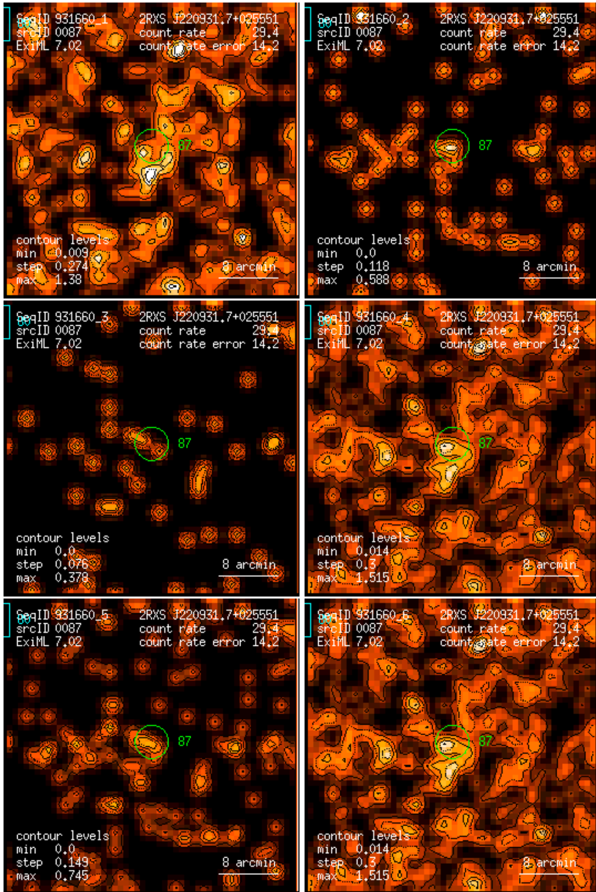
Figure 87: RASS 931660: detection 0087: band rate images, Gaussian filter: (1) PSPC channels 11 – 41, (2) 52 – 90, (3) 91 – 201, (4) 11 – 235, (5) 52 – 201, (6) 11 – 201. Broad band rates in counts/ks. Band rate contour levels in counts/ks/arcmin 2 .
