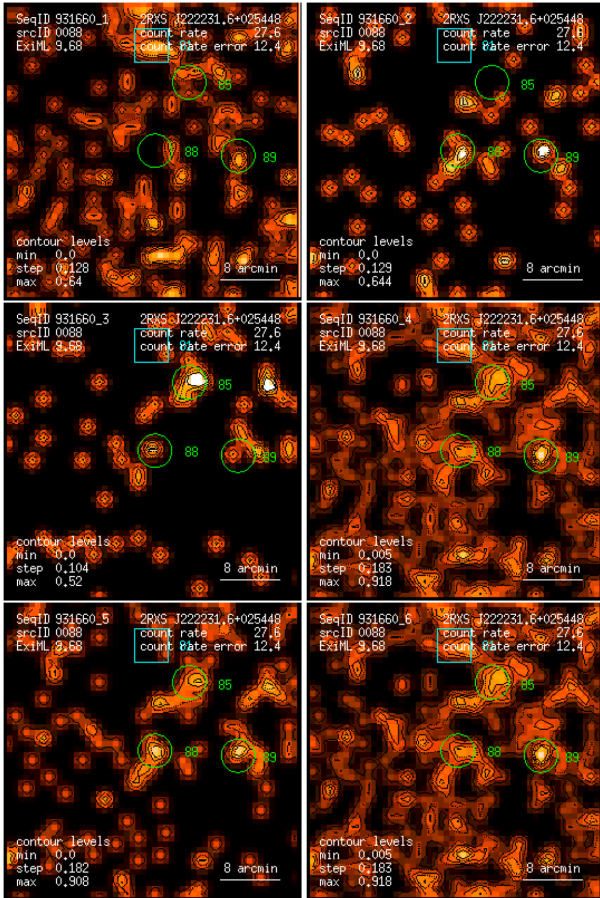
Figure 88: RASS 931660: detection 0088: band rate images, Gaussian filter: (1) PSPC channels 11 – 41, (2) 52 – 90, (3) 91 – 201, (4) 11 – 235, (5) 52 – 201, (6) 11 – 201. Broad band rates in counts/ks. Band rate contour levels in counts/ks/arcmin 2 .
