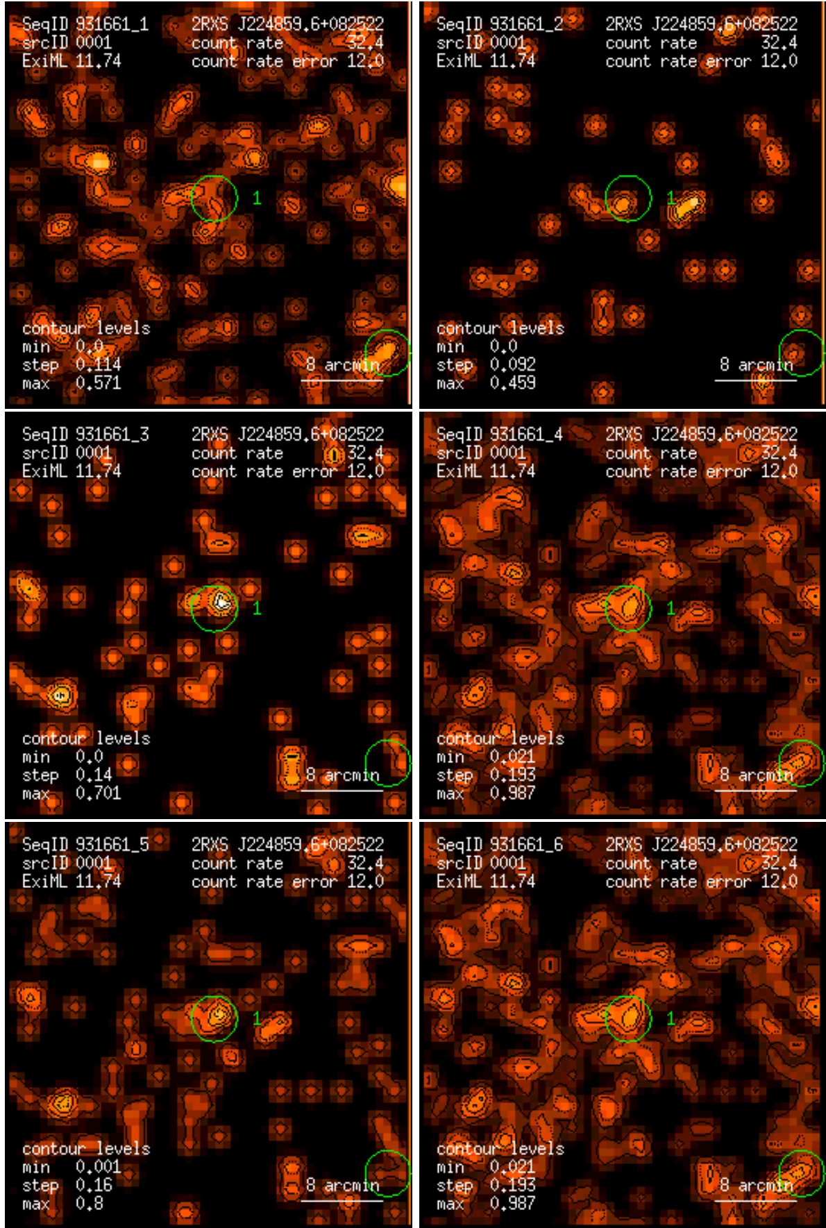
Figure 1: RASS 931661: detection 0001: band rate images, Gaussian filter: (1) PSPC channels 11 – 41, (2) 52 – 90, (3) 91 – 201, (4) 11 – 235, (5) 52 – 201, (6) 11 – 201. Broad band rates in counts/ks. Band rate contour levels in counts/ks/arcmin 2 .
