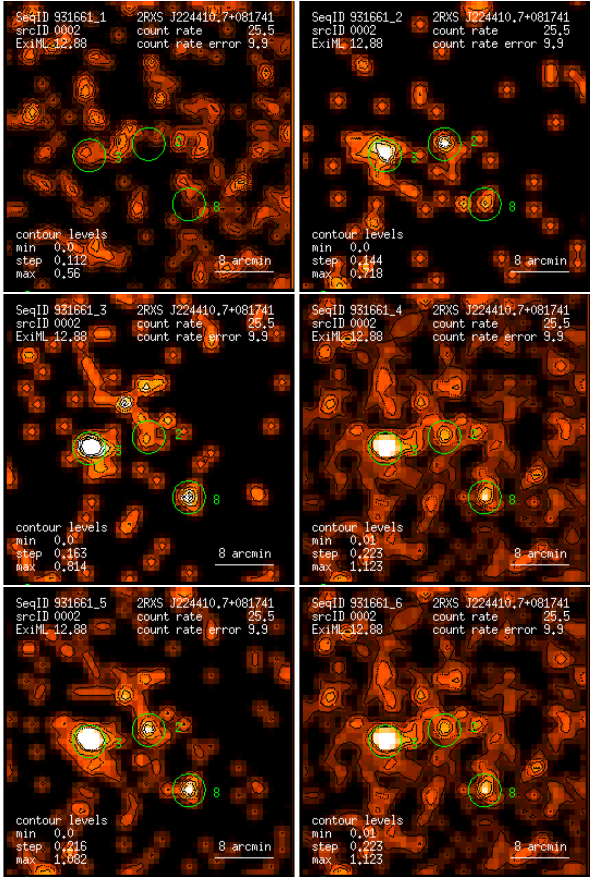
Figure 2: RASS 931661: detection 0002: band rate images, Gaussian filter: (1) PSPC channels 11 – 41, (2) 52 – 90, (3) 91 – 201, (4) 11 – 235, (5) 52 – 201, (6) 11 – 201. Broad band rates in counts/ks. Band rate contour levels in counts/ks/arcmin 2 .
