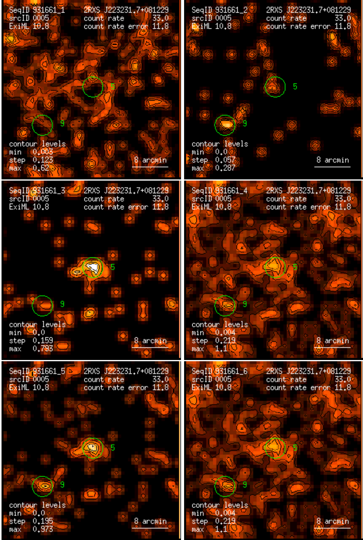
Figure 5: RASS 931661: detection 0005: band rate images, Gaussian filter: (1) PSPC channels 11 – 41, (2) 52 – 90, (3) 91 – 201, (4) 11 – 235, (5) 52 – 201, (6) 11 – 201. Broad band rates in counts/ks. Band rate contour levels in counts/ks/arcmin 2 .
