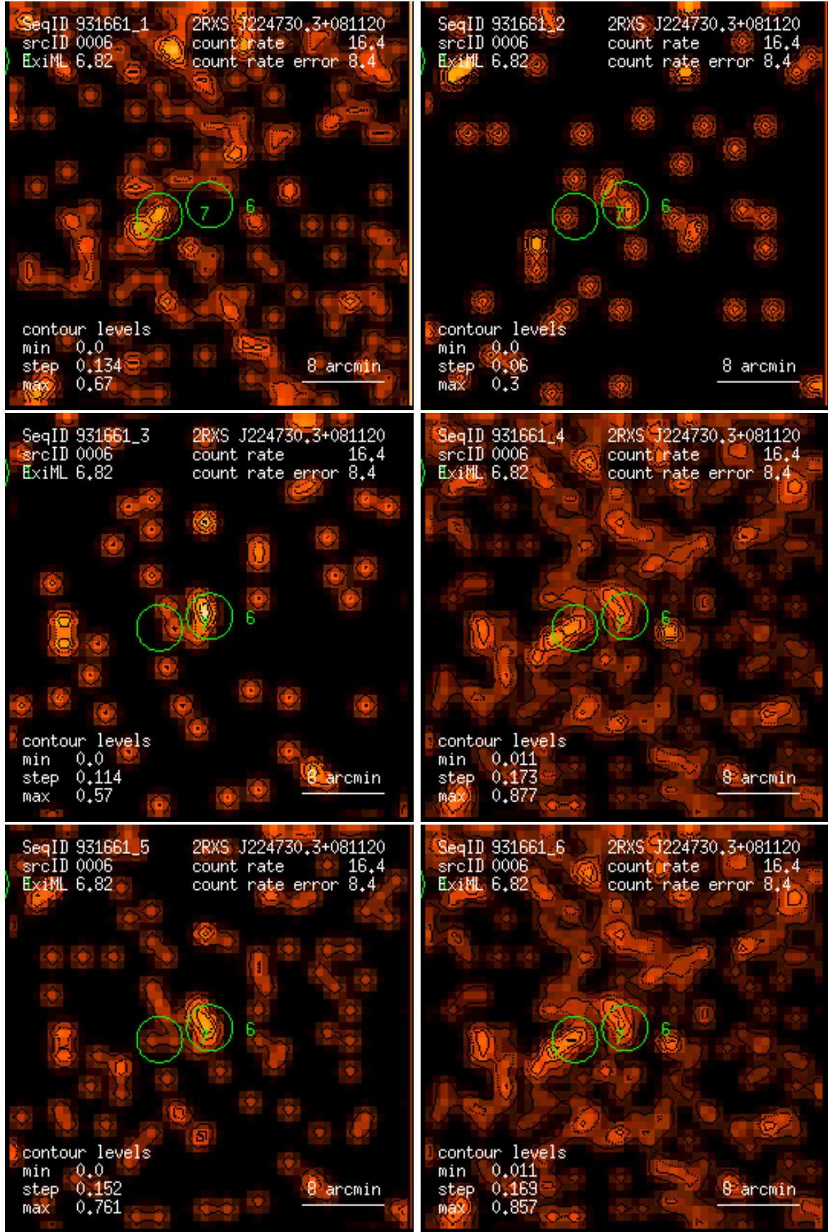
Figure 6: RASS 931661: detection 0006: band rate images, Gaussian filter: (1) PSPC channels 11 – 41, (2) 52 – 90, (3) 91 – 201, (4) 11 – 235, (5) 52 – 201, (6) 11 – 201. Broad band rates in counts/ks. Band rate contour levels in counts/ks/arcmin 2 .
