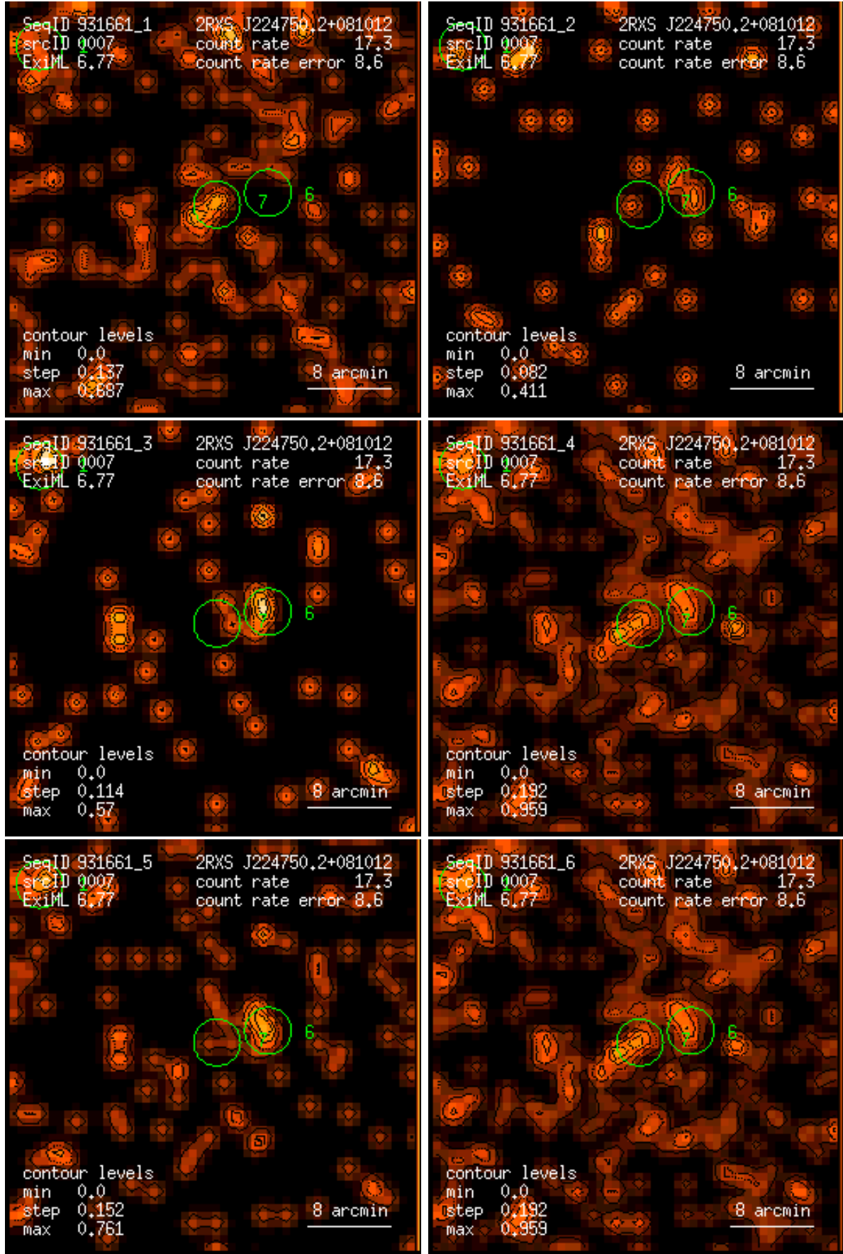
Figure 7: RASS 931661: detection 0007: band rate images, Gaussian filter: (1) PSPC channels 11 – 41, (2) 52 – 90, (3) 91 – 201, (4) 11 – 235, (5) 52 – 201, (6) 11 – 201. Broad band rates in counts/ks. Band rate contour levels in counts/ks/arcmin 2 .
