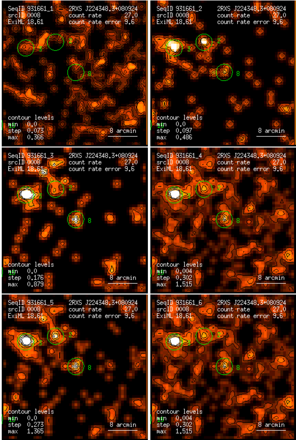
Figure 8: RASS 931661: detection 0008: band rate images, Gaussian filter: (1) PSPC channels 11 – 41, (2) 52 – 90, (3) 91 – 201, (4) 11 – 235, (5) 52 – 201, (6) 11 – 201. Broad band rates in counts/ks. Band rate contour levels in counts/ks/arcmin 2 .
