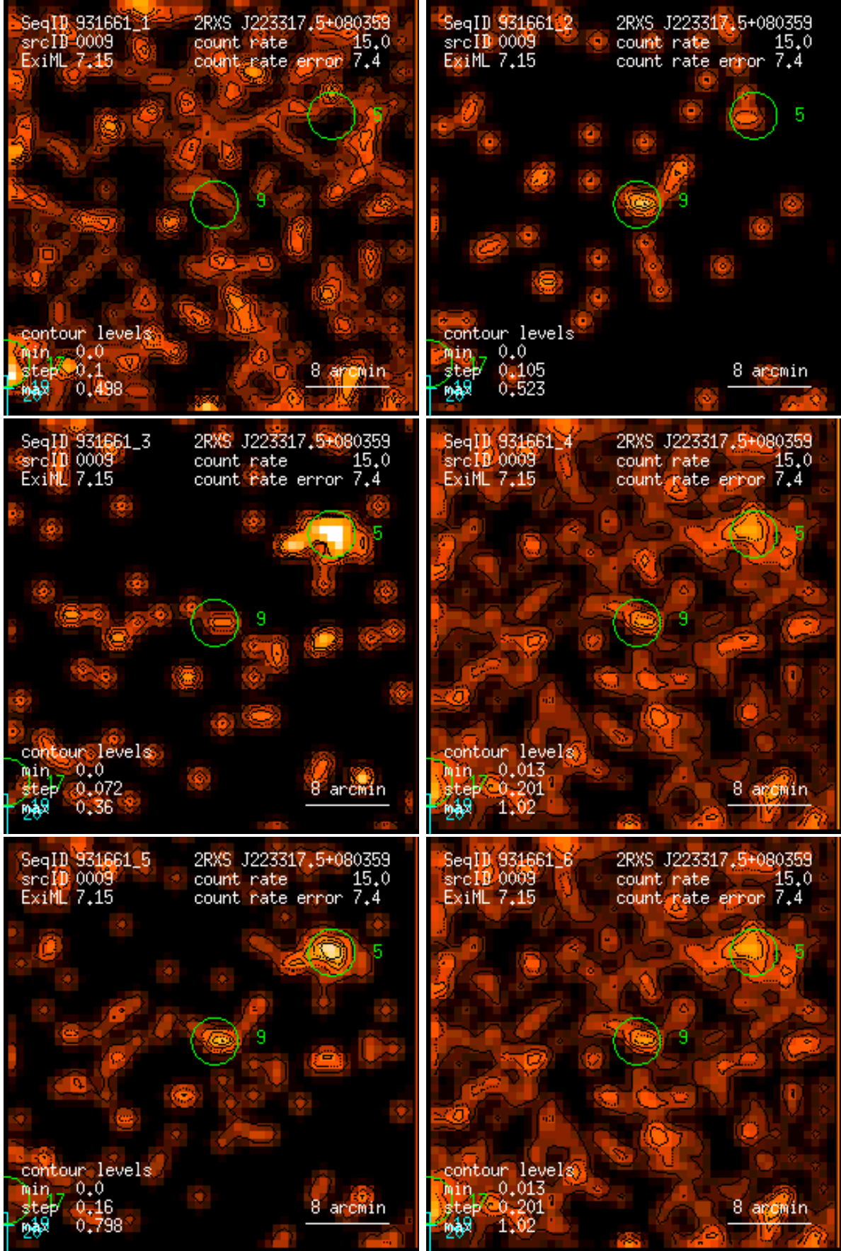
Figure 9: RASS 931661: detection 0009: band rate images, Gaussian filter: (1) PSPC channels 11 – 41, (2) 52 – 90, (3) 91 – 201, (4) 11 – 235, (5) 52 – 201, (6) 11 – 201. Broad band rates in counts/ks. Band rate contour levels in counts/ks/arcmin 2 .
