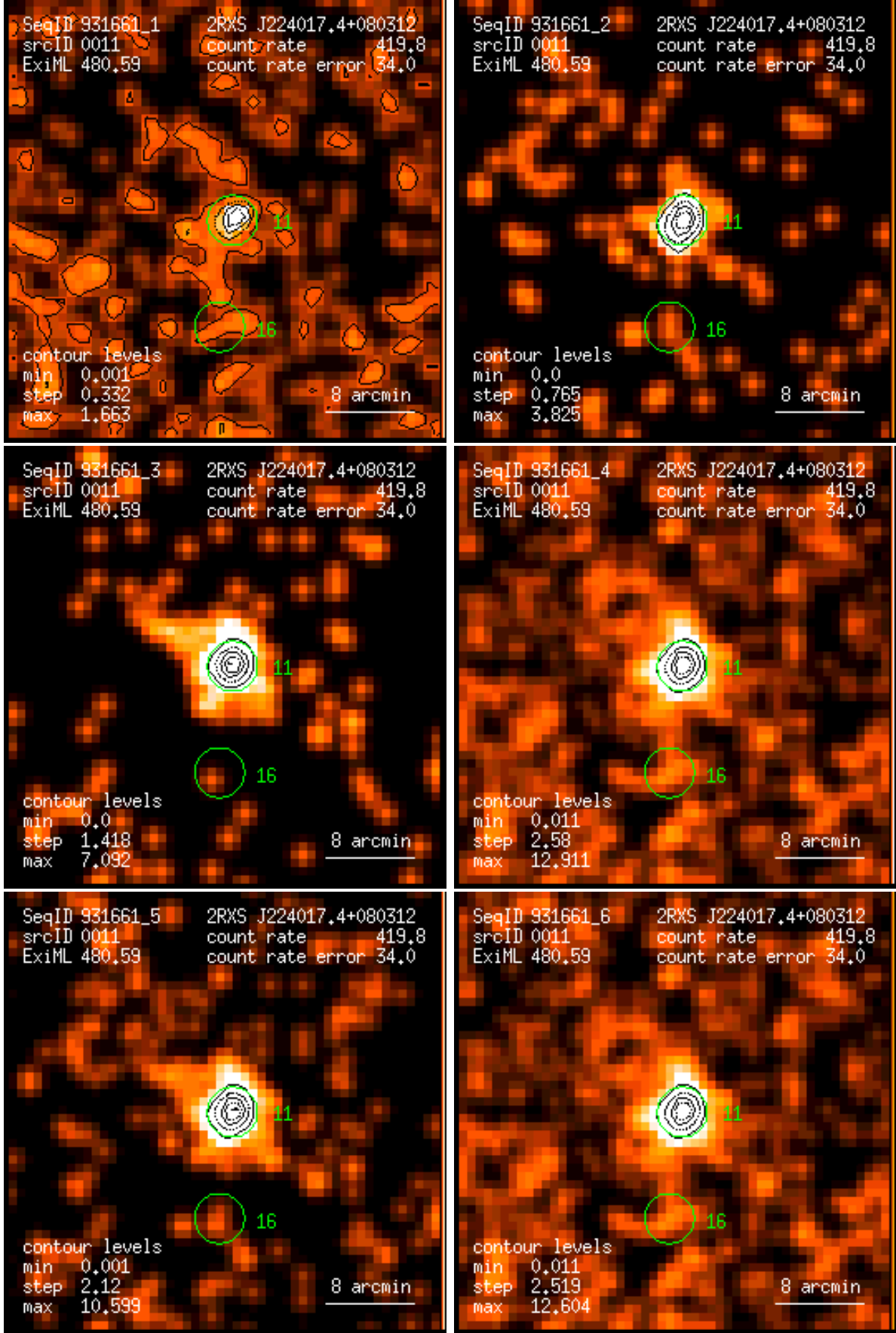
Figure 11: RASS 931661: detection 0011: band rate images, Gaussian filter: (1) PSPC channels 11 – 41, (2) 52 – 90, (3) 91 – 201, (4) 11 – 235, (5) 52 – 201, (6) 11 – 201. Broad band rates in counts/ks. Band rate contour levels in counts/ks/arcmin 2 .
