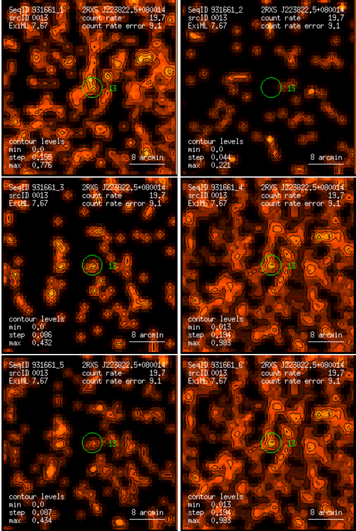
Figure 13: RASS 931661: detection 0013: band rate images, Gaussian filter: (1) PSPC channels 11 – 41, (2) 52 – 90, (3) 91 – 201, (4) 11 – 235, (5) 52 – 201, (6) 11 – 201. Broad band rates in counts/ks. Band rate contour levels in counts/ks/arcmin 2 .
