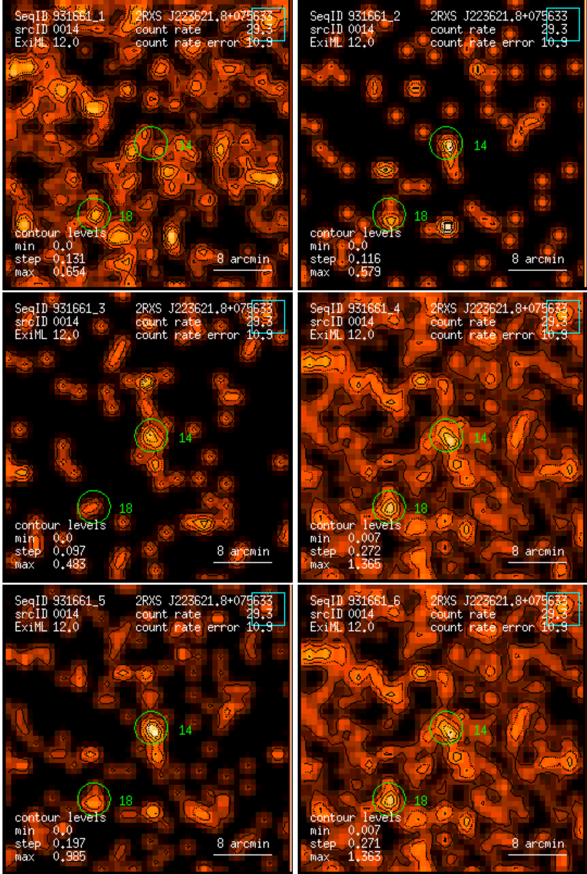
Figure 14: RASS 931661: detection 0014: band rate images, Gaussian filter: (1) PSPC channels 11 – 41, (2) 52 – 90, (3) 91 – 201, (4) 11 – 235, (5) 52 – 201, (6) 11 – 201. Broad band rates in counts/ks. Band rate contour levels in counts/ks/arcmin 2 .
