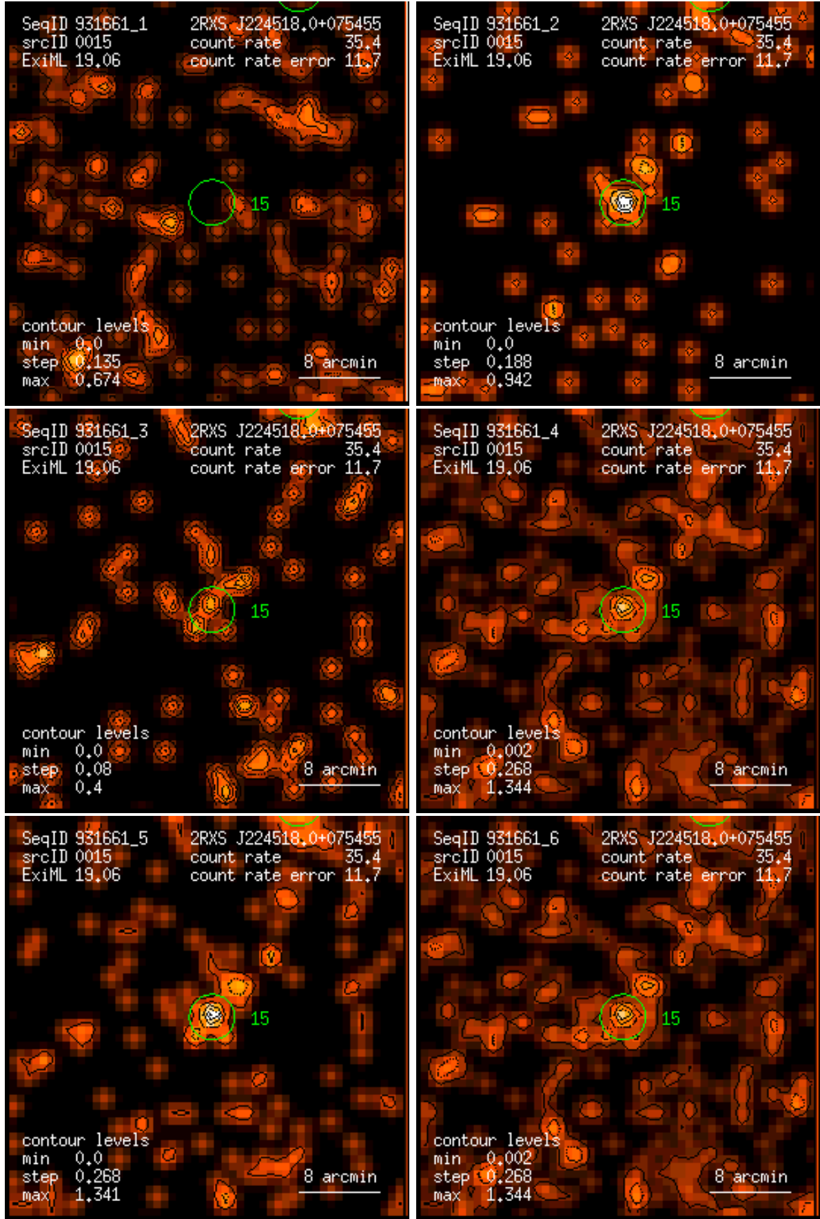
Figure 15: RASS 931661: detection 0015: band rate images, Gaussian filter: (1) PSPC channels 11 – 41, (2) 52 – 90, (3) 91 – 201, (4) 11 – 235, (5) 52 – 201, (6) 11 – 201. Broad band rates in counts/ks. Band rate contour levels in counts/ks/arcmin 2 .
