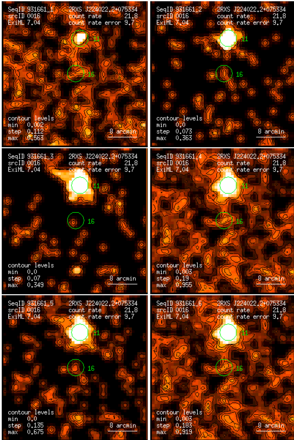
Figure 16: RASS 931661: detection 0016: band rate images, Gaussian filter: (1) PSPC channels 11 – 41, (2) 52 – 90, (3) 91 – 201, (4) 11 – 235, (5) 52 – 201, (6) 11 – 201. Broad band rates in counts/ks. Band rate contour levels in counts/ks/arcmin 2 .
