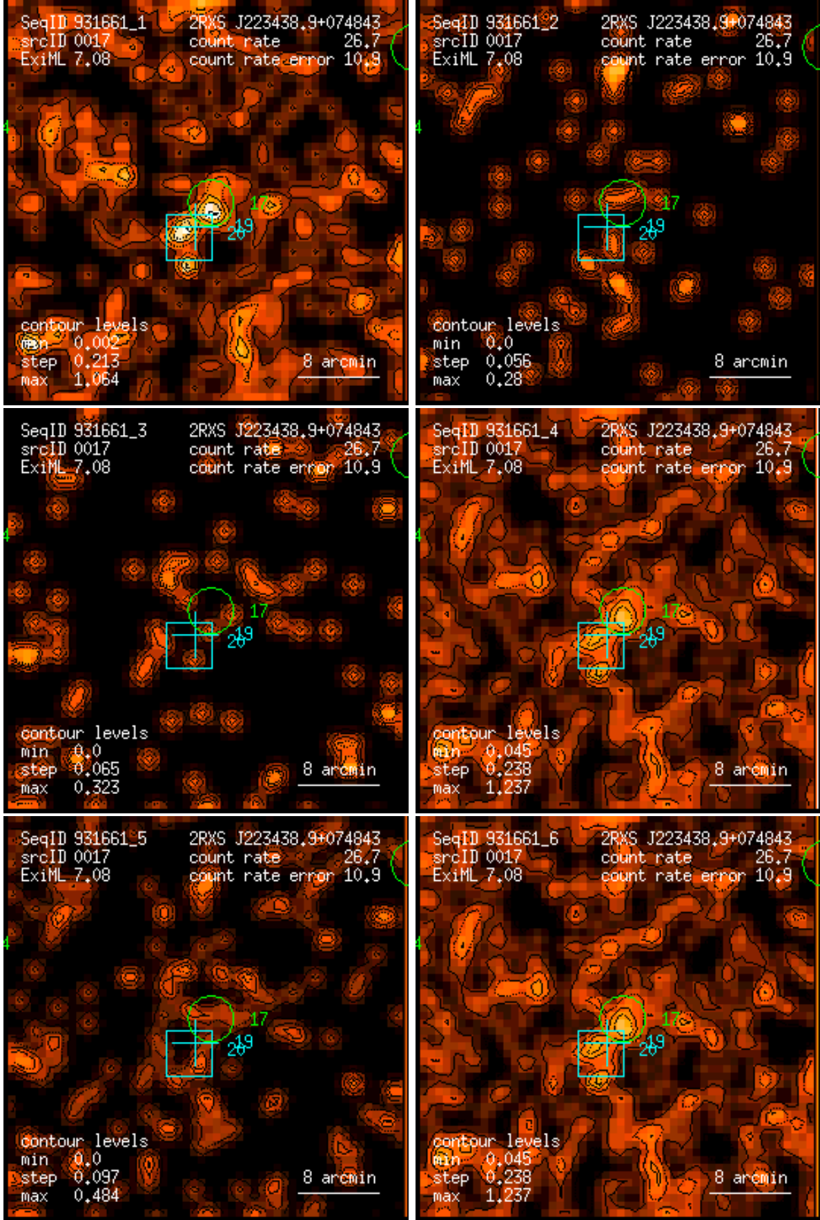
Figure 17: RASS 931661: detection 0017: band rate images, Gaussian filter: (1) PSPC channels 11 – 41, (2) 52 – 90, (3) 91 – 201, (4) 11 – 235, (5) 52 – 201, (6) 11 – 201. Broad band rates in counts/ks. Band rate contour levels in counts/ks/arcmin 2 .
