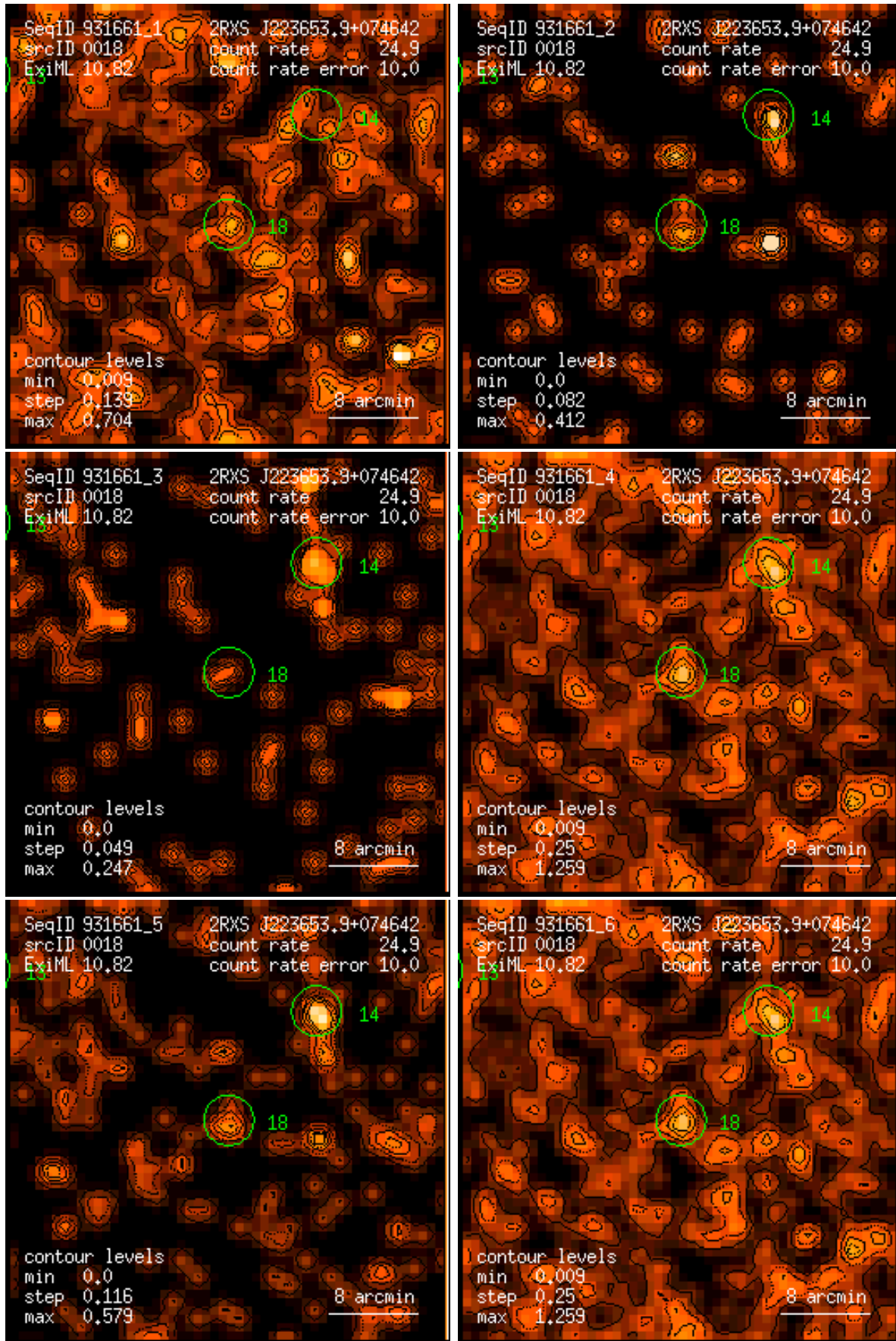
Figure 18: RASS 931661: detection 0018: band rate images, Gaussian filter: (1) PSPC channels 11 – 41, (2) 52 – 90, (3) 91 – 201, (4) 11 – 235, (5) 52 – 201, (6) 11 – 201. Broad band rates in counts/ks. Band rate contour levels in counts/ks/arcmin 2 .
