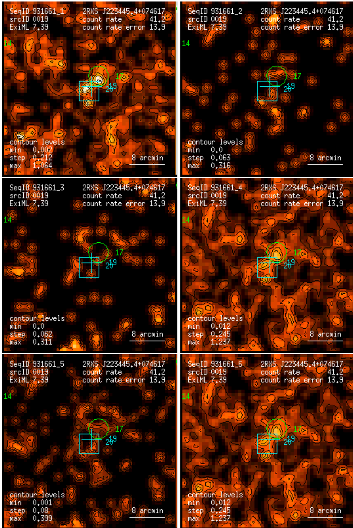
Figure 19: RASS 931661: detection 0019: band rate images, Gaussian filter: (1) PSPC channels 11 – 41, (2) 52 – 90, (3) 91 – 201, (4) 11 – 235, (5) 52 – 201, (6) 11 – 201. Broad band rates in counts/ks. Band rate contour levels in counts/ks/arcmin 2 .
