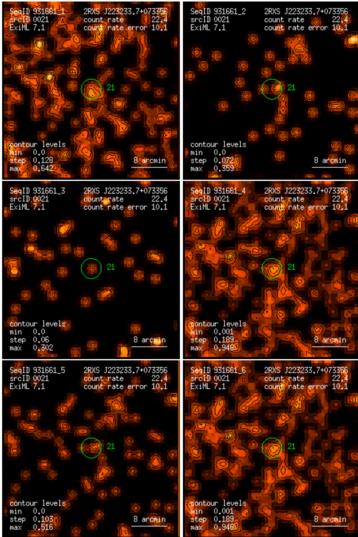
Figure 21: RASS 931661: detection 0021: band rate images, Gaussian filter: (1) PSPC channels 11 – 41, (2) 52 – 90, (3) 91 – 201, (4) 11 – 235, (5) 52 – 201, (6) 11 – 201. Broad band rates in counts/ks. Band rate contour levels in counts/ks/arcmin 2 .
