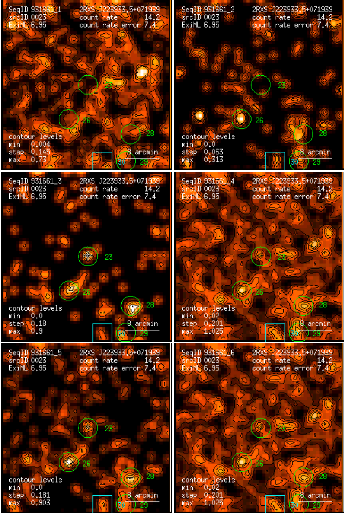
Figure 23: RASS 931661: detection 0023: band rate images, Gaussian filter: (1) PSPC channels 11 – 41, (2) 52 – 90, (3) 91 – 201, (4) 11 – 235, (5) 52 – 201, (6) 11 – 201. Broad band rates in counts/ks. Band rate contour levels in counts/ks/arcmin 2 .
