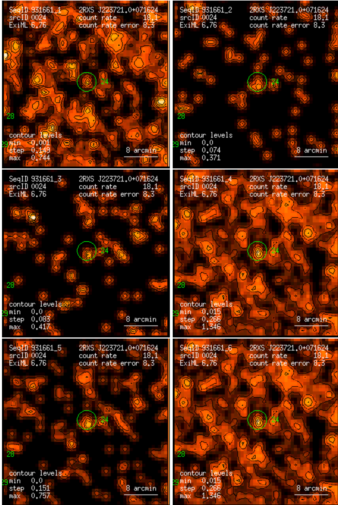
Figure 24: RASS 931661: detection 0024: band rate images, Gaussian filter: (1) PSPC channels 11 – 41, (2) 52 – 90, (3) 91 – 201, (4) 11 – 235, (5) 52 – 201, (6) 11 – 201. Broad band rates in counts/ks. Band rate contour levels in counts/ks/arcmin 2 .
