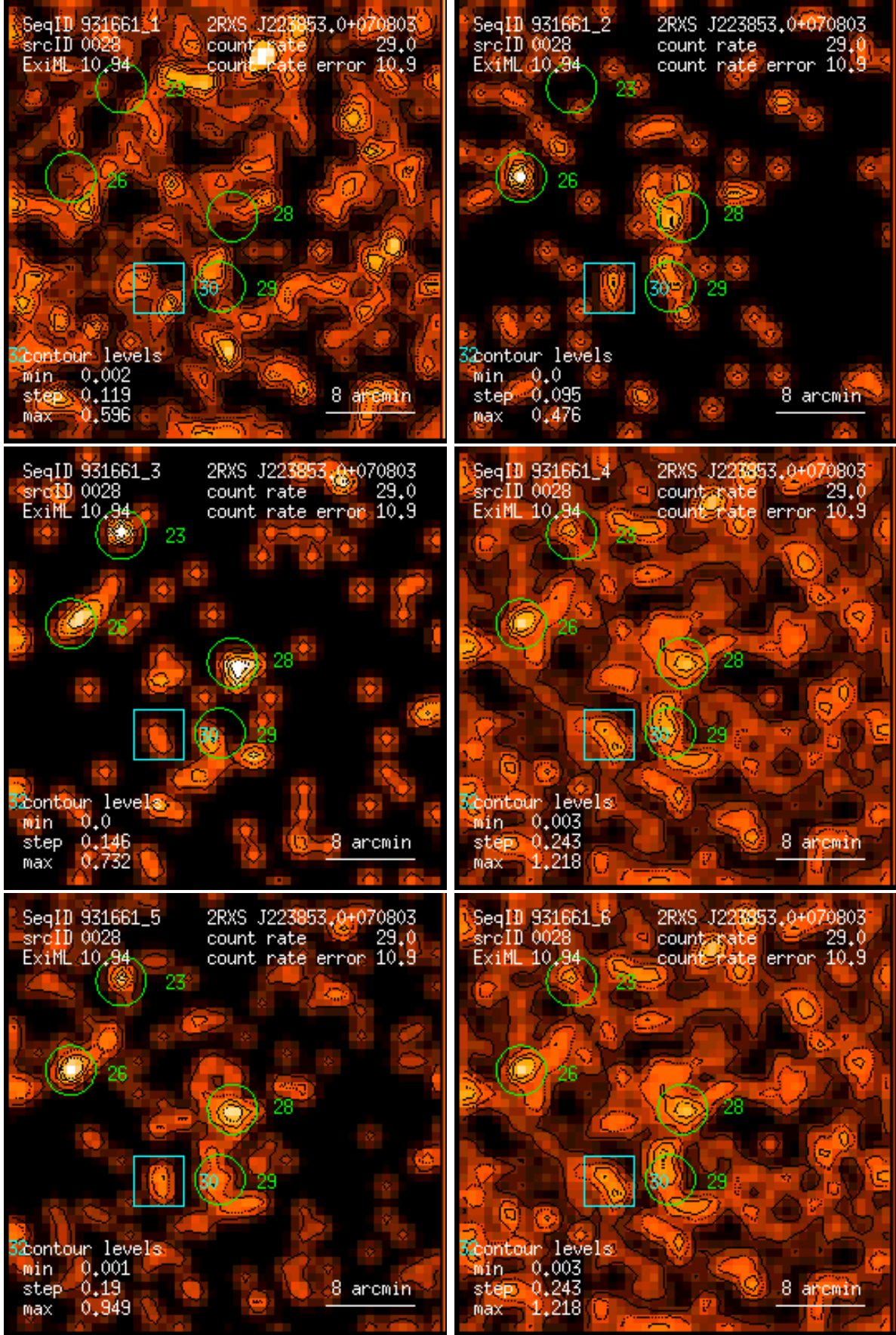
Figure 28: RASS 931661: detection 0028: band rate images, Gaussian filter: (1) PSPC channels 11 – 41, (2) 52 – 90, (3) 91 – 201, (4) 11 – 235, (5) 52 – 201, (6) 11 – 201. Broad band rates in counts/ks. Band rate contour levels in counts/ks/arcmin 2 .
