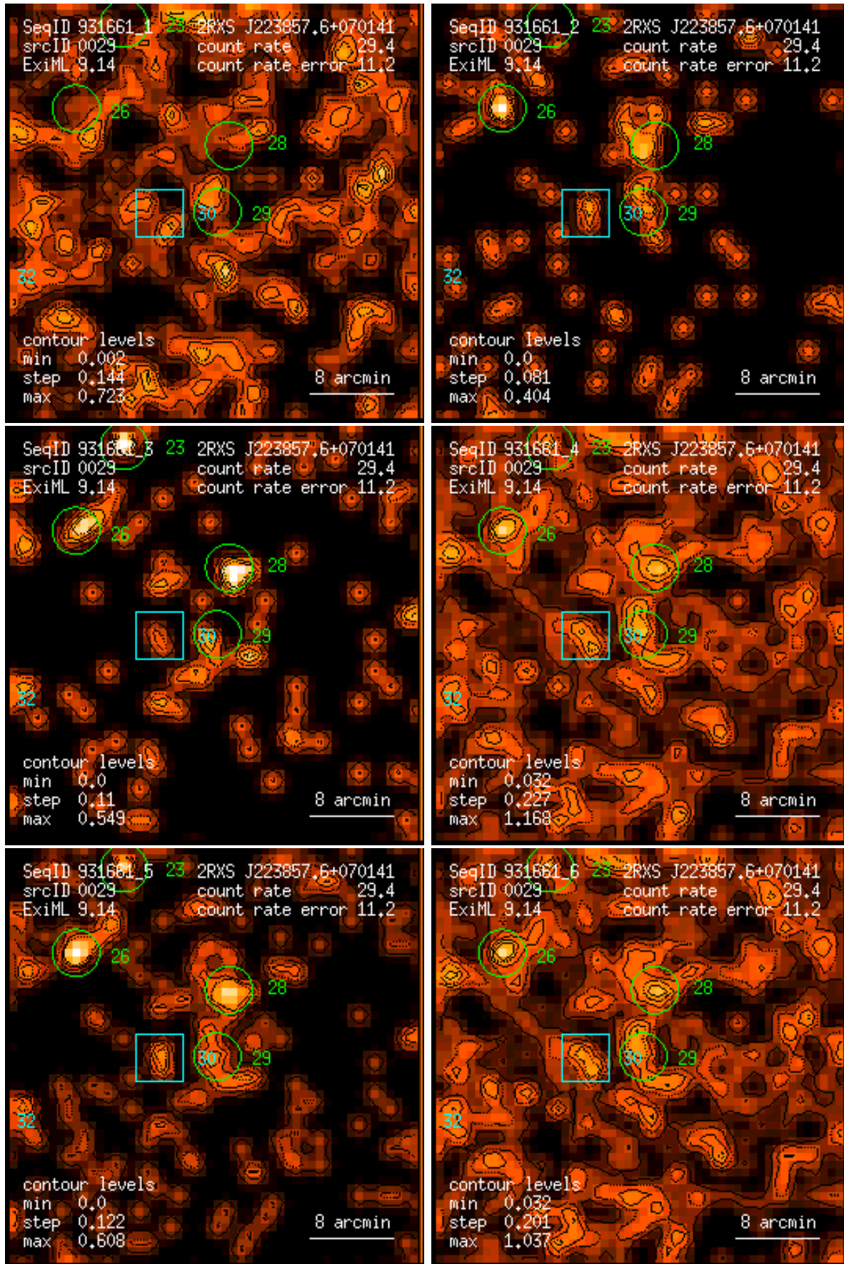
Figure 29: RASS 931661: detection 0029: band rate images, Gaussian filter: (1) PSPC channels 11 – 41, (2) 52 – 90, (3) 91 – 201, (4) 11 – 235, (5) 52 – 201, (6) 11 – 201. Broad band rates in counts/ks. Band rate contour levels in counts/ks/arcmin 2 .
