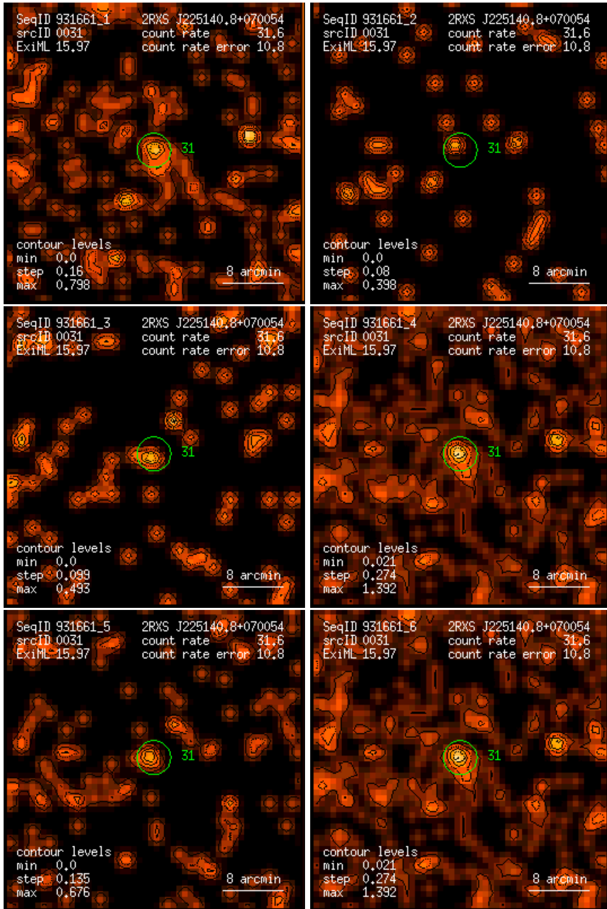
Figure 31: RASS 931661: detection 0031: band rate images, Gaussian filter: (1) PSPC channels 11 – 41, (2) 52 – 90, (3) 91 – 201, (4) 11 – 235, (5) 52 – 201, (6) 11 – 201. Broad band rates in counts/ks. Band rate contour levels in counts/ks/arcmin 2 .
