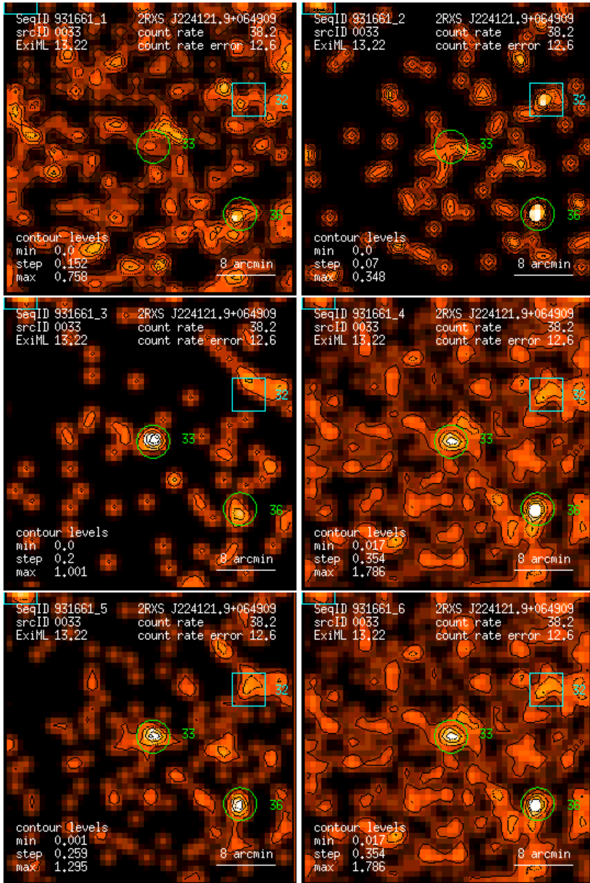
Figure 33: RASS 931661: detection 0033: band rate images, Gaussian filter: (1) PSPC channels 11 – 41, (2) 52 – 90, (3) 91 – 201, (4) 11 – 235, (5) 52 – 201, (6) 11 – 201. Broad band rates in counts/ks. Band rate contour levels in counts/ks/arcmin 2 .
