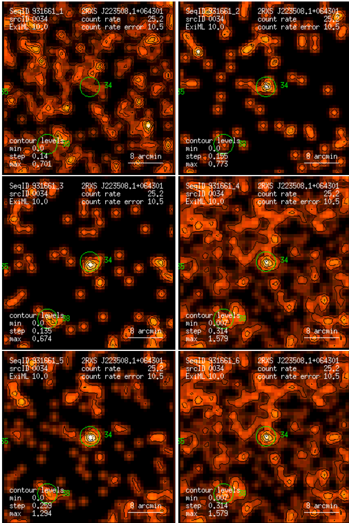
Figure 34: RASS 931661: detection 0034: band rate images, Gaussian filter: (1) PSPC channels 11 – 41, (2) 52 – 90, (3) 91 – 201, (4) 11 – 235, (5) 52 – 201, (6) 11 – 201. Broad band rates in counts/ks. Band rate contour levels in counts/ks/arcmin 2 .
