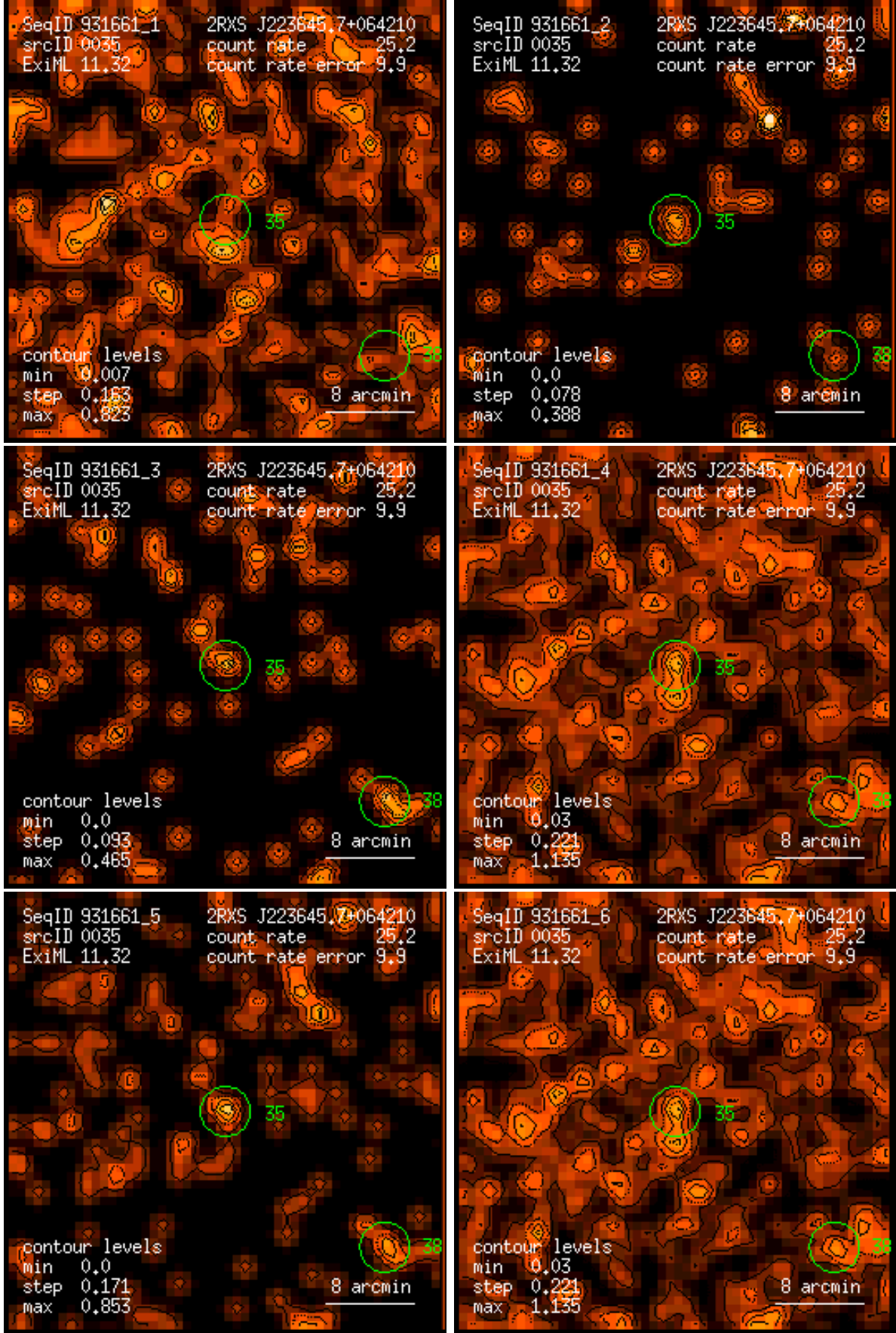
Figure 35: RASS 931661: detection 0035: band rate images, Gaussian filter: (1) PSPC channels 11 – 41, (2) 52 – 90, (3) 91 – 201, (4) 11 – 235, (5) 52 – 201, (6) 11 – 201. Broad band rates in counts/ks. Band rate contour levels in counts/ks/arcmin 2 .
