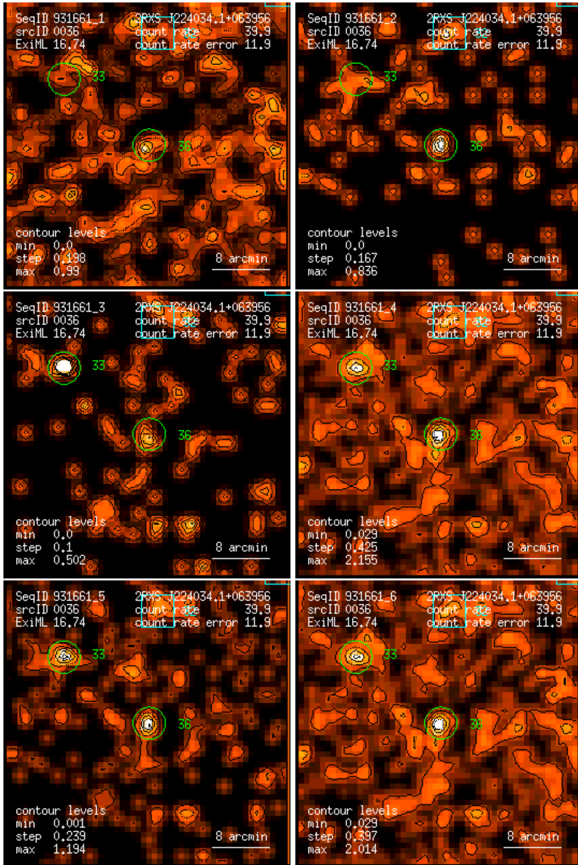
Figure 36: RASS 931661: detection 0036: band rate images, Gaussian filter: (1) PSPC channels 11 – 41, (2) 52 – 90, (3) 91 – 201, (4) 11 – 235, (5) 52 – 201, (6) 11 – 201. Broad band rates in counts/ks. Band rate contour levels in counts/ks/arcmin 2 .
