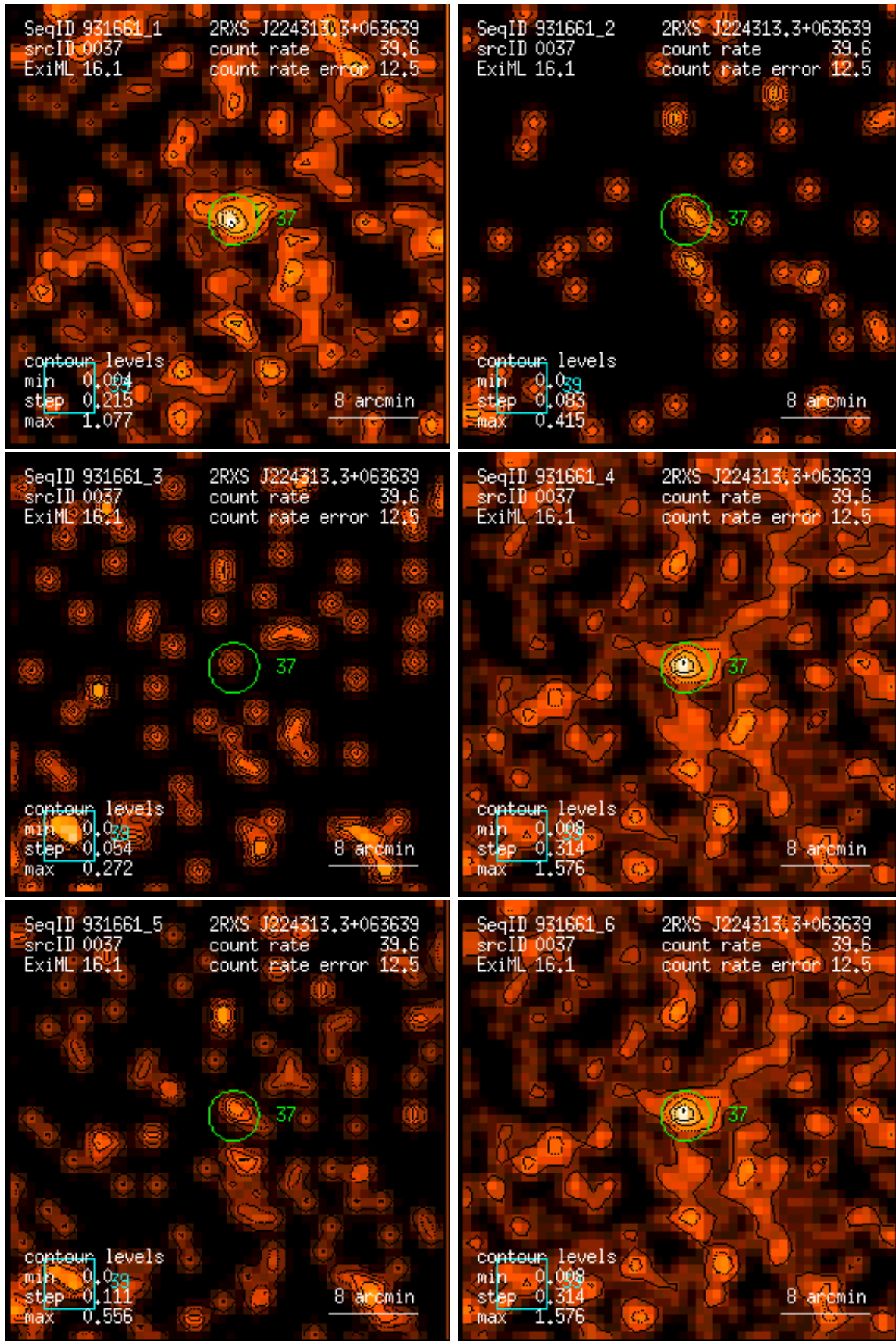
Figure 37: RASS 931661: detection 0037: band rate images, Gaussian filter: (1) PSPC channels 11 – 41, (2) 52 – 90, (3) 91 – 201, (4) 11 – 235, (5) 52 – 201, (6) 11 – 201. Broad band rates in counts/ks. Band rate contour levels in counts/ks/arcmin 2 .
