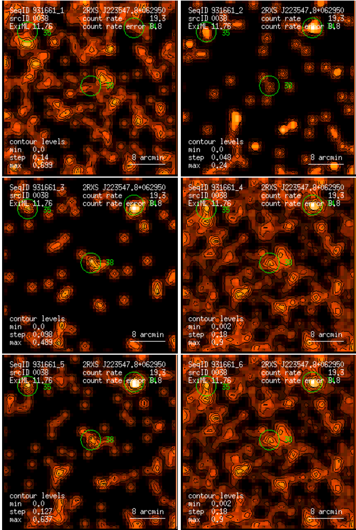
Figure 38: RASS 931661: detection 0038: band rate images, Gaussian filter: (1) PSPC channels 11 – 41, (2) 52 – 90, (3) 91 – 201, (4) 11 – 235, (5) 52 – 201, (6) 11 – 201. Broad band rates in counts/ks. Band rate contour levels in counts/ks/arcmin 2 .
