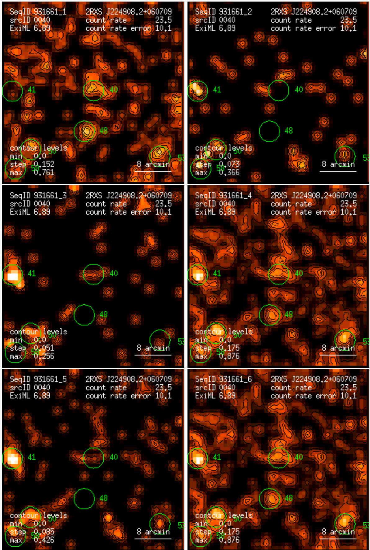
Figure 40: RASS 931661: detection 0040: band rate images, Gaussian filter: (1) PSPC channels 11 – 41, (2) 52 – 90, (3) 91 – 201, (4) 11 – 235, (5) 52 – 201, (6) 11 – 201. Broad band rates in counts/ks. Band rate contour levels in counts/ks/arcmin 2 .
