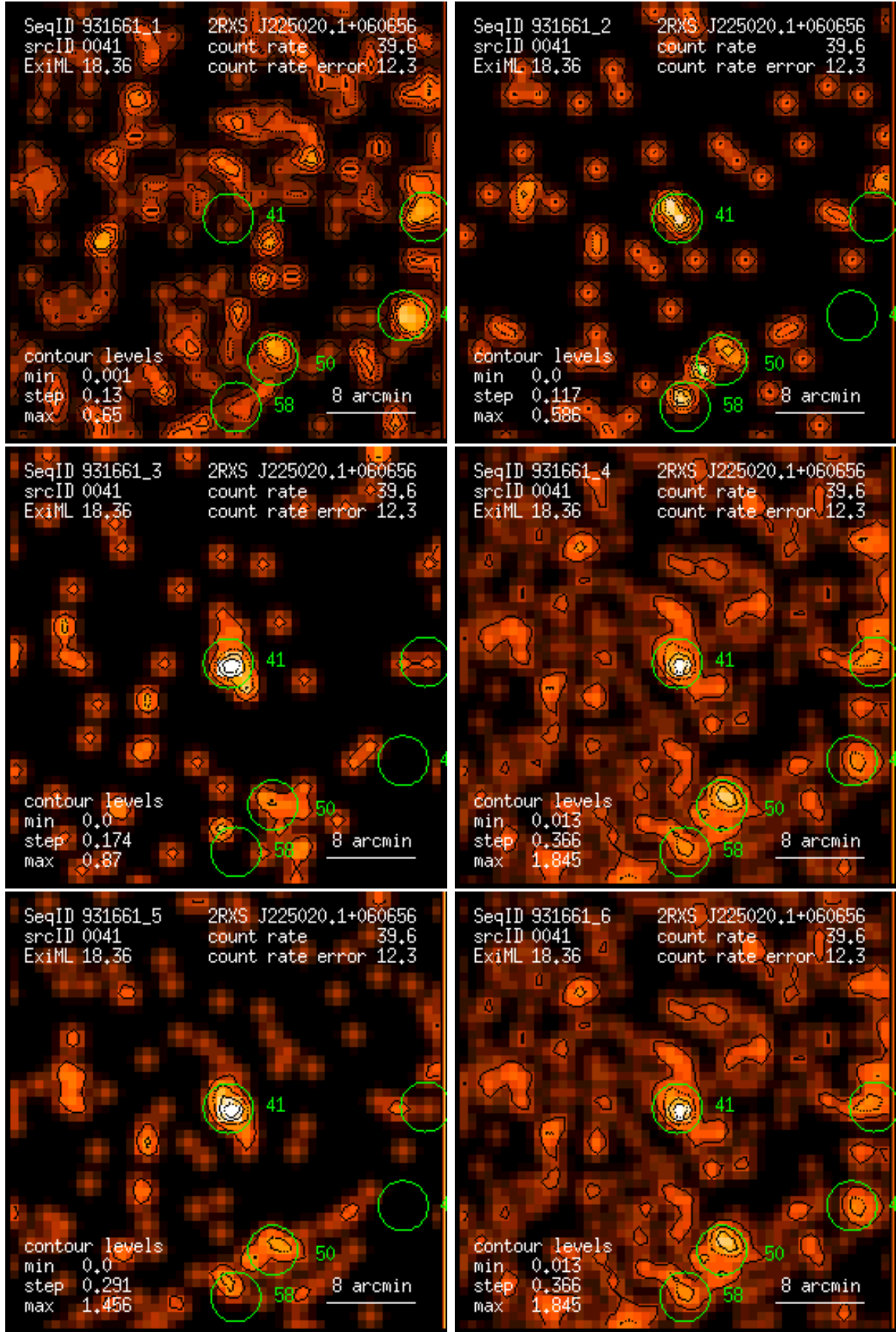
Figure 41: RASS 931661: detection 0041: band rate images, Gaussian filter: (1) PSPC channels 11 – 41, (2) 52 – 90, (3) 91 – 201, (4) 11 – 235, (5) 52 – 201, (6) 11 – 201. Broad band rates in counts/ks. Band rate contour levels in counts/ks/arcmin 2 .
