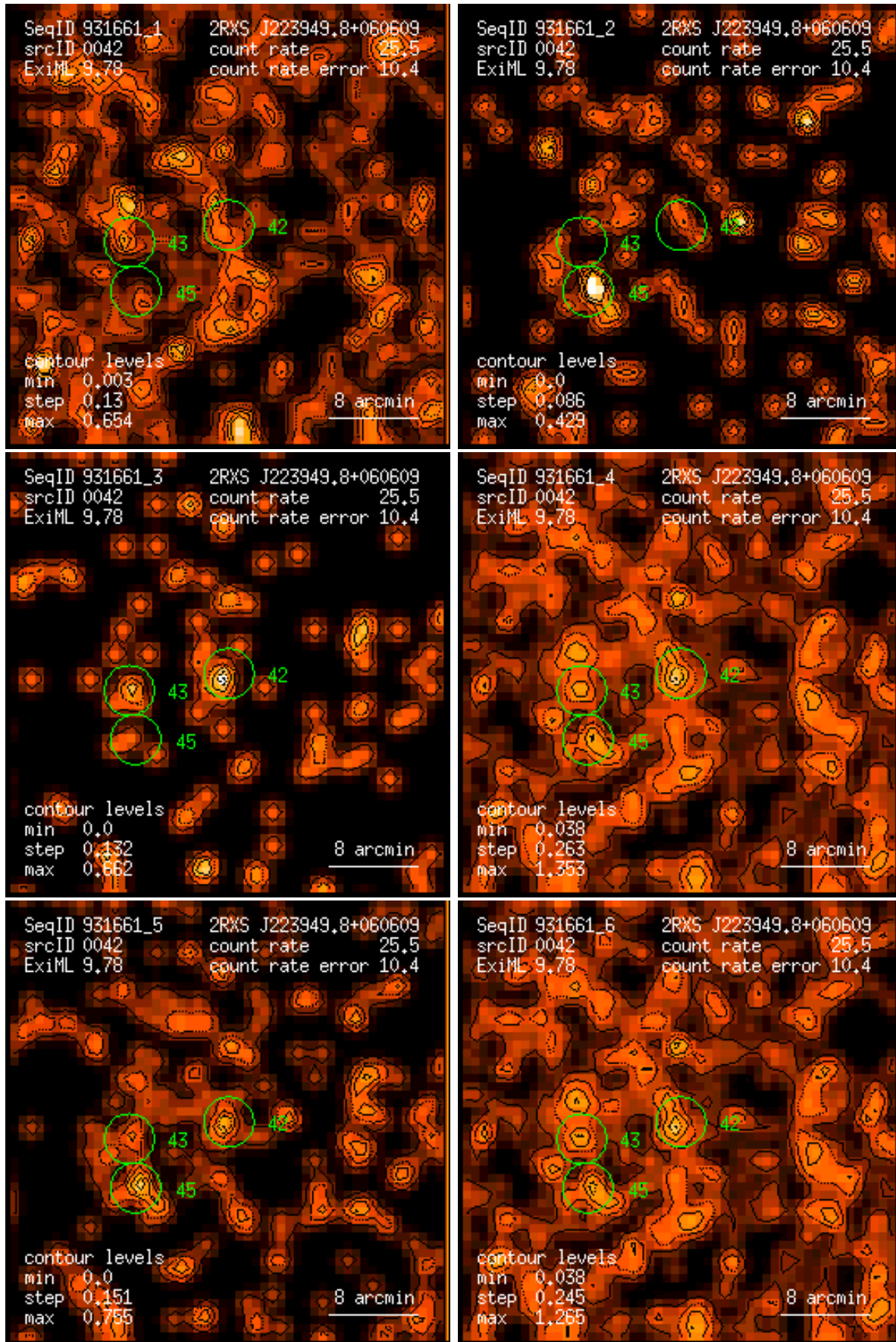
Figure 42: RASS 931661: detection 0042: band rate images, Gaussian filter: (1) PSPC channels 11 – 41, (2) 52 – 90, (3) 91 – 201, (4) 11 – 235, (5) 52 – 201, (6) 11 – 201. Broad band rates in counts/ks. Band rate contour levels in counts/ks/arcmin 2 .
