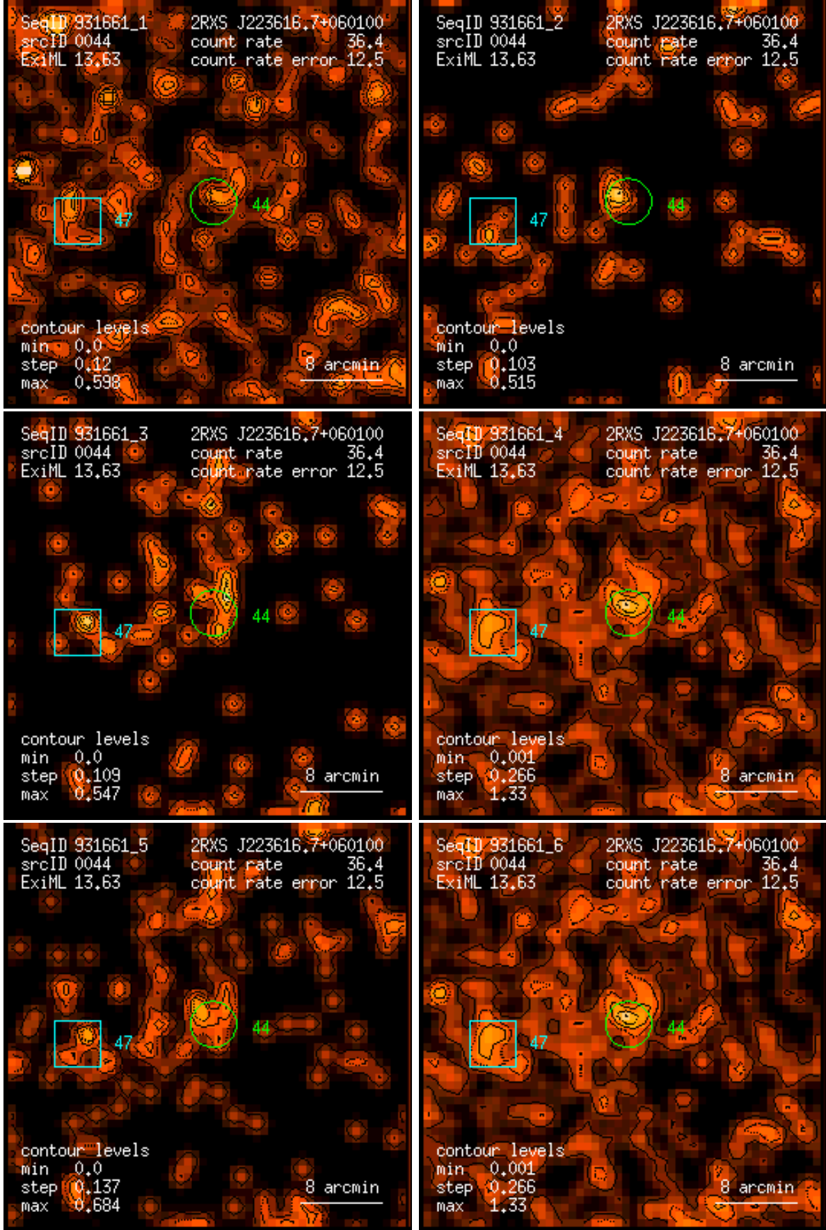
Figure 44: RASS 931661: detection 0044: band rate images, Gaussian filter: (1) PSPC channels 11 – 41, (2) 52 – 90, (3) 91 – 201, (4) 11 – 235, (5) 52 – 201, (6) 11 – 201. Broad band rates in counts/ks. Band rate contour levels in counts/ks/arcmin 2 .
