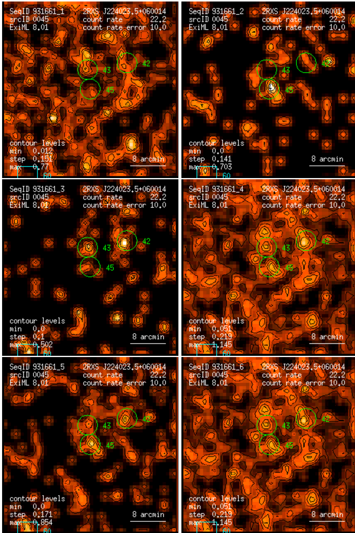
Figure 45: RASS 931661: detection 0045: band rate images, Gaussian filter: (1) PSPC channels 11 – 41, (2) 52 – 90, (3) 91 – 201, (4) 11 – 235, (5) 52 – 201, (6) 11 – 201. Broad band rates in counts/ks. Band rate contour levels in counts/ks/arcmin 2 .
