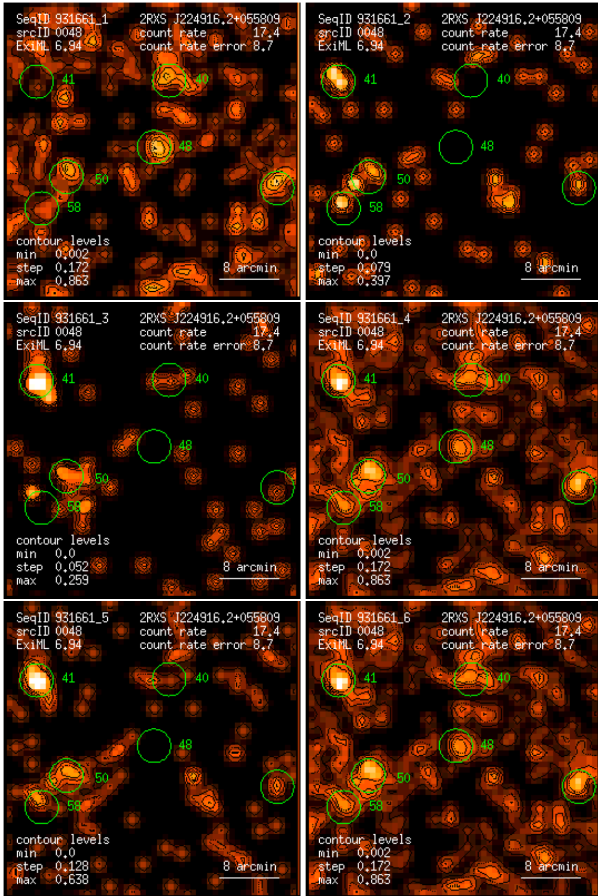
Figure 48: RASS 931661: detection 0048: band rate images, Gaussian filter: (1) PSPC channels 11 – 41, (2) 52 – 90, (3) 91 – 201, (4) 11 – 235, (5) 52 – 201, (6) 11 – 201. Broad band rates in counts/ks. Band rate contour levels in counts/ks/arcmin 2 .
