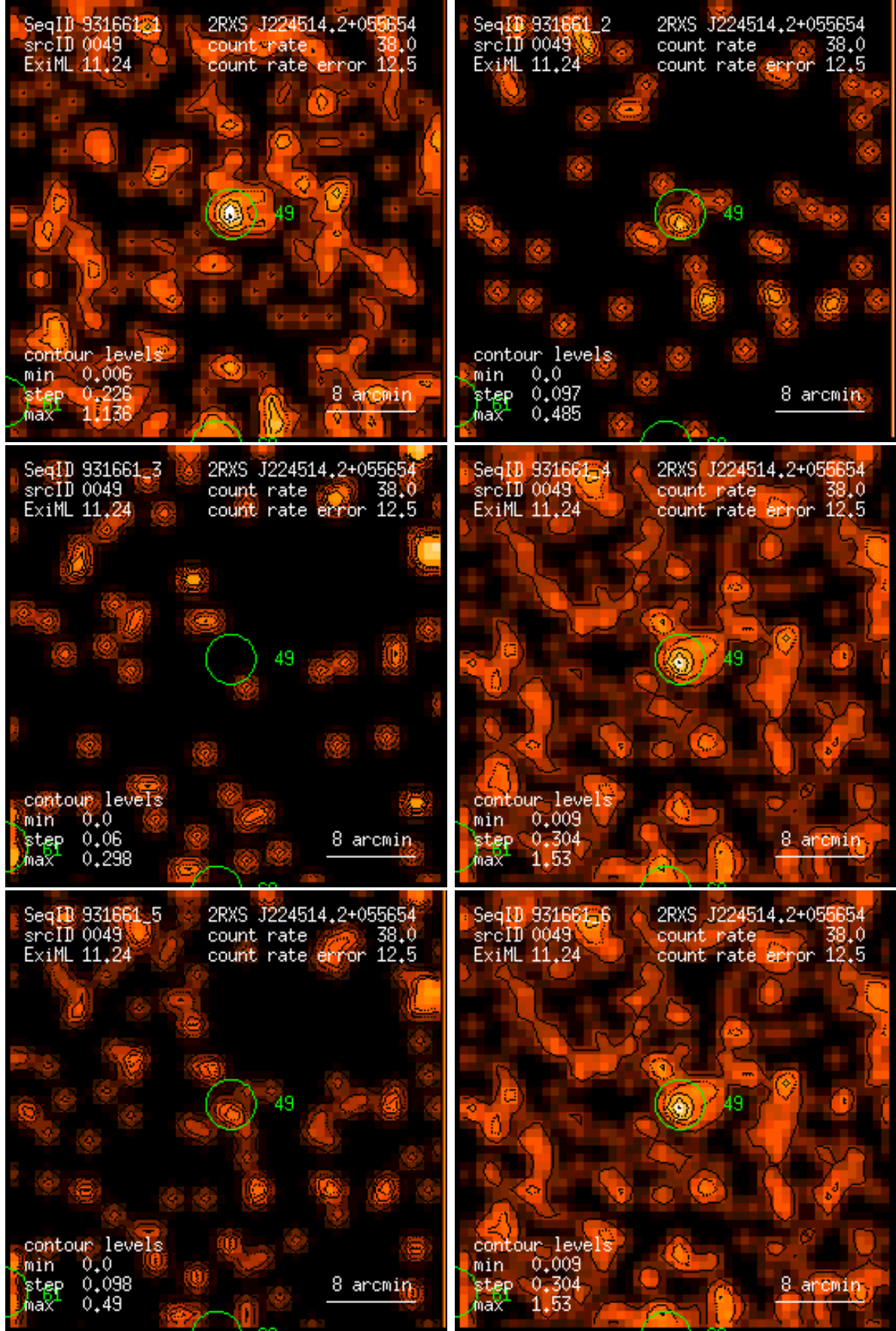
Figure 49: RASS 931661: detection 0049: band rate images, Gaussian filter: (1) PSPC channels 11 – 41, (2) 52 – 90, (3) 91 – 201, (4) 11 – 235, (5) 52 – 201, (6) 11 – 201. Broad band rates in counts/ks. Band rate contour levels in counts/ks/arcmin 2 .
