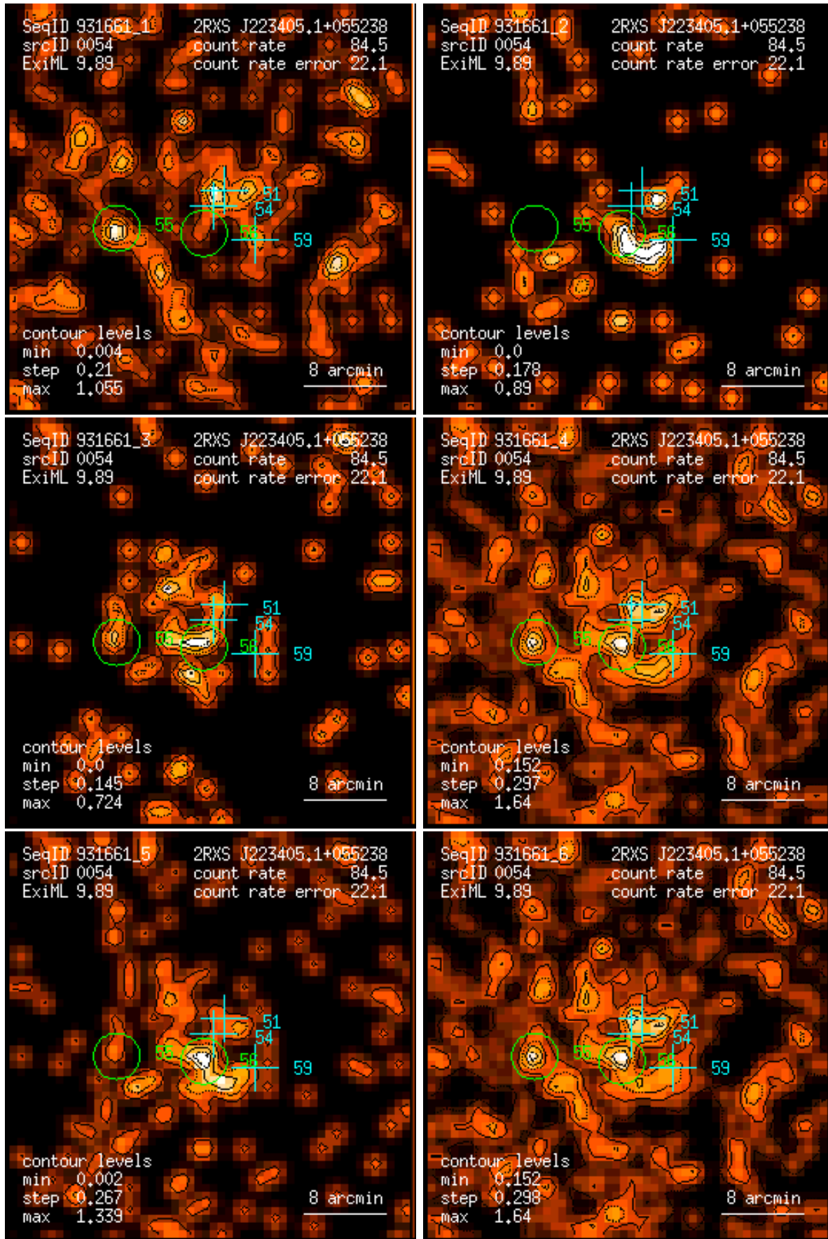
Figure 54: RASS 931661: detection 0054: band rate images, Gaussian filter: (1) PSPC channels 11 – 41, (2) 52 – 90, (3) 91 – 201, (4) 11 – 235, (5) 52 – 201, (6) 11 – 201. Broad band rates in counts/ks. Band rate contour levels in counts/ks/arcmin 2 .
