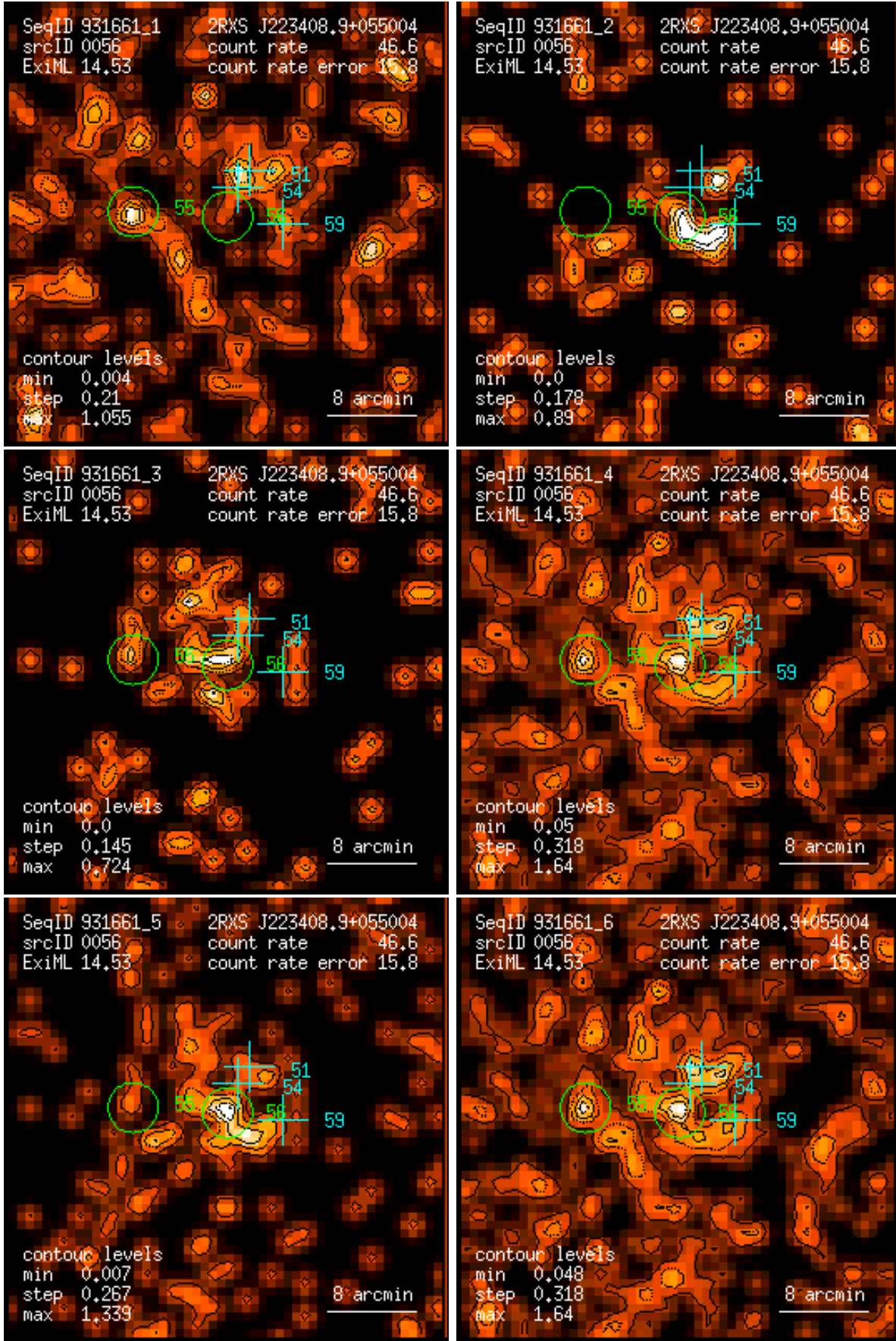
Figure 56: RASS 931661: detection 0056: band rate images, Gaussian filter: (1) PSPC channels 11 – 41, (2) 52 – 90, (3) 91 – 201, (4) 11 – 235, (5) 52 – 201, (6) 11 – 201. Broad band rates in counts/ks. Band rate contour levels in counts/ks/arcmin 2 .
