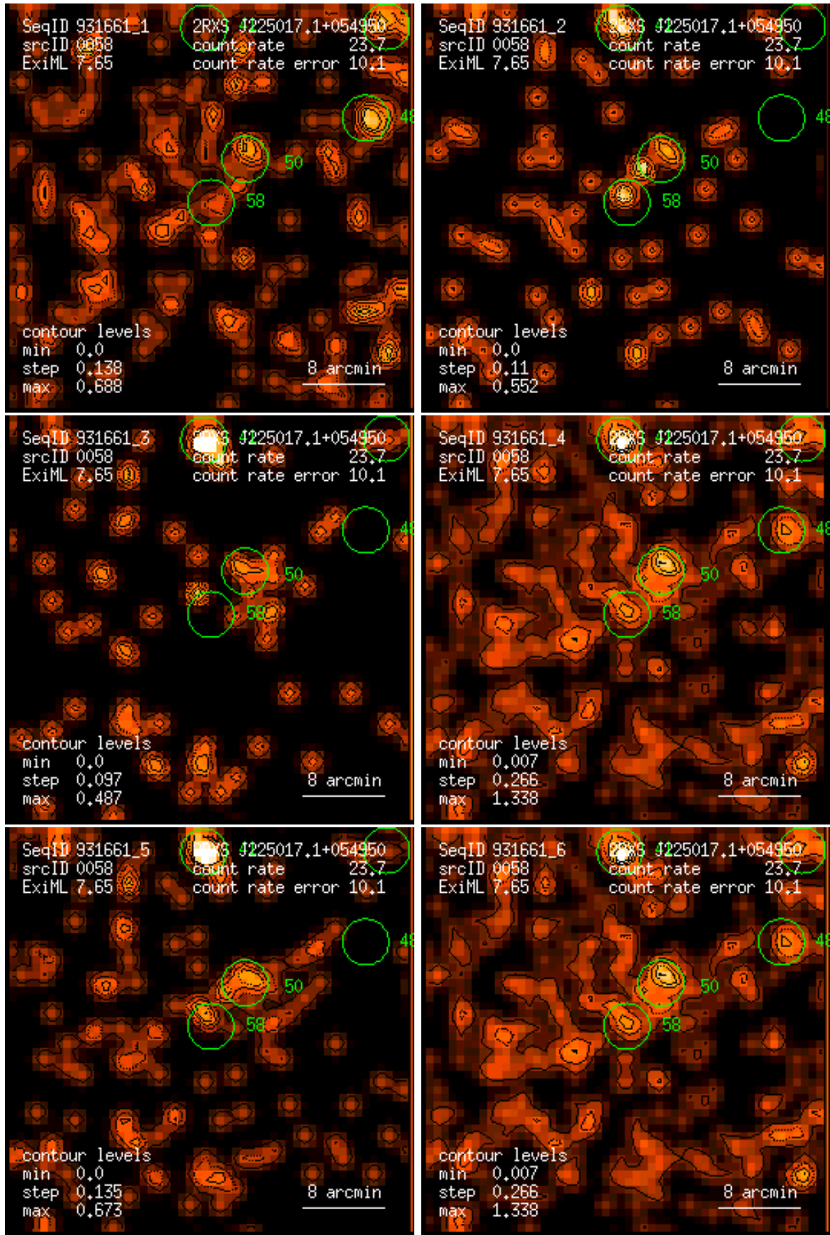
Figure 58: RASS 931661: detection 0058: band rate images, Gaussian filter: (1) PSPC channels 11 – 41, (2) 52 – 90, (3) 91 – 201, (4) 11 – 235, (5) 52 – 201, (6) 11 – 201. Broad band rates in counts/ks. Band rate contour levels in counts/ks/arcmin 2 .
