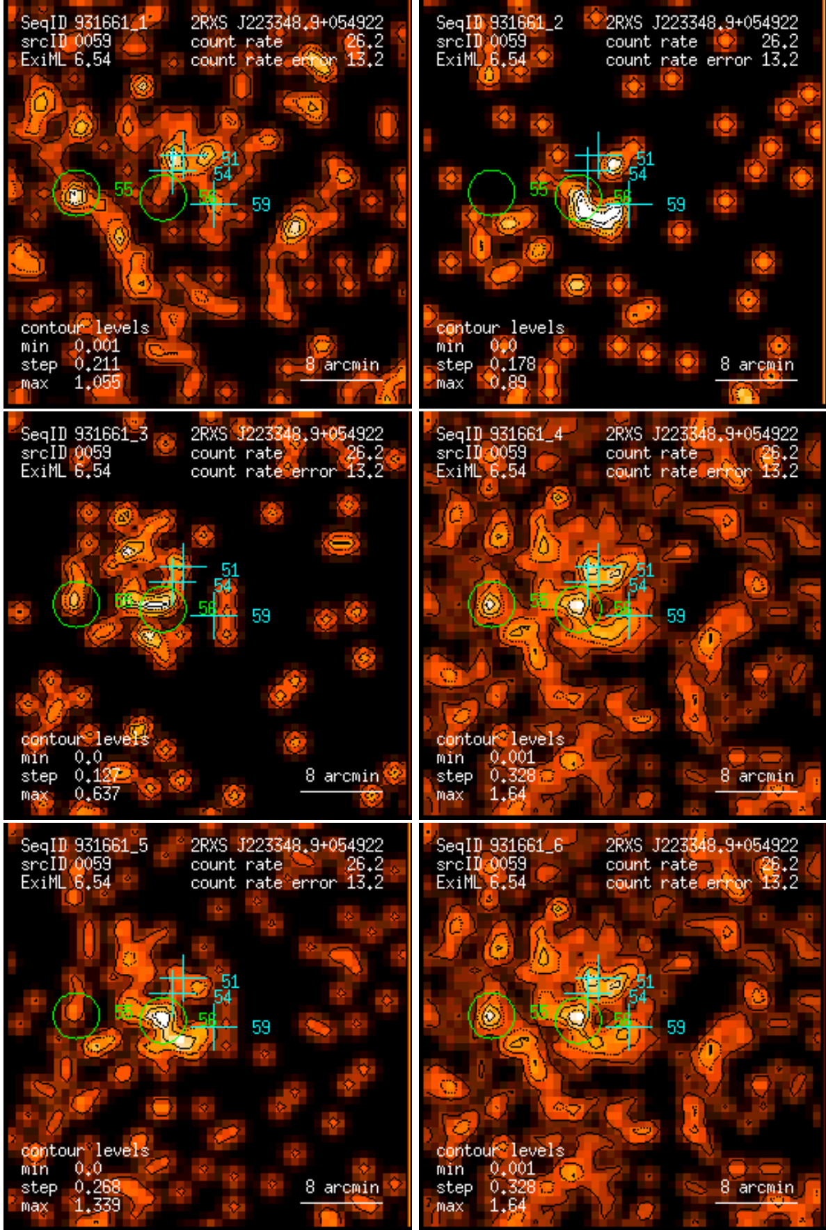
Figure 59: RASS 931661: detection 0059: band rate images, Gaussian filter: (1) PSPC channels 11 – 41, (2) 52 – 90, (3) 91 – 201, (4) 11 – 235, (5) 52 – 201, (6) 11 – 201. Broad band rates in counts/ks. Band rate contour levels in counts/ks/arcmin 2 .
