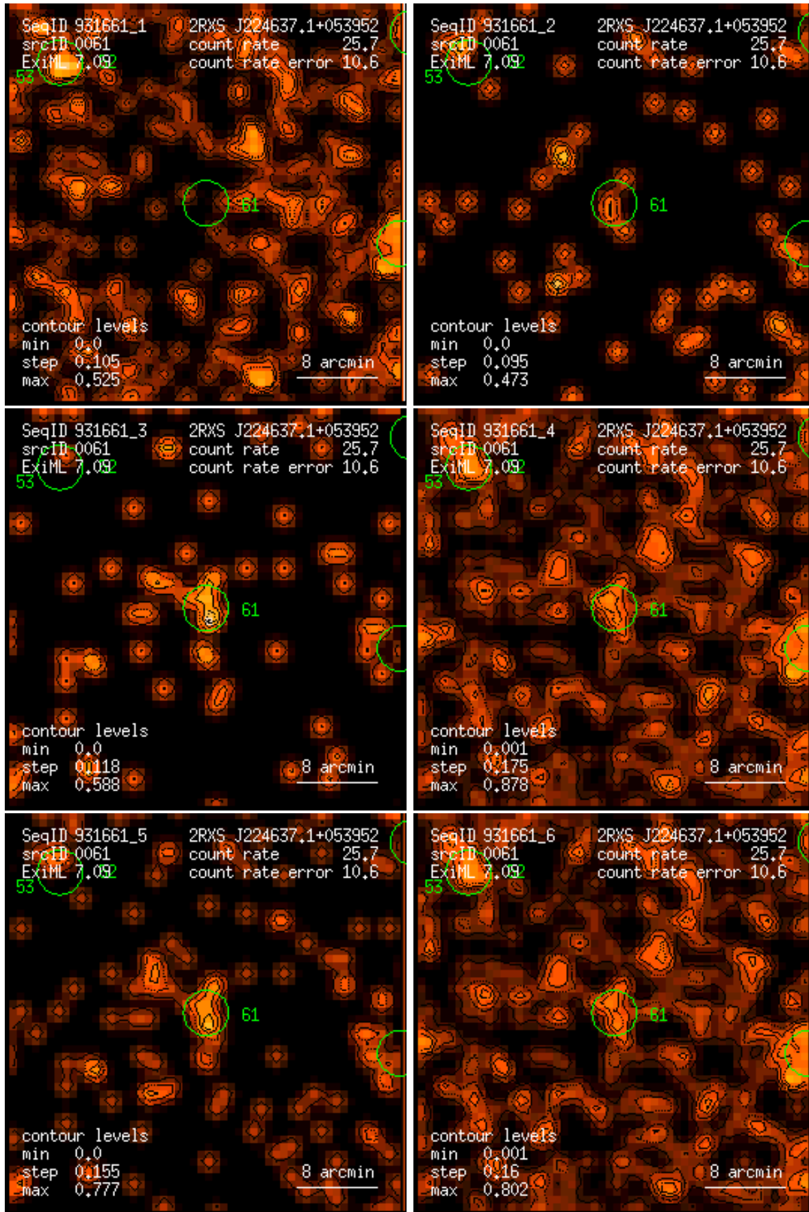
Figure 61: RASS 931661: detection 0061: band rate images, Gaussian filter: (1) PSPC channels 11 – 41, (2) 52 – 90, (3) 91 – 201, (4) 11 – 235, (5) 52 – 201, (6) 11 – 201. Broad band rates in counts/ks. Band rate contour levels in counts/ks/arcmin 2 .
