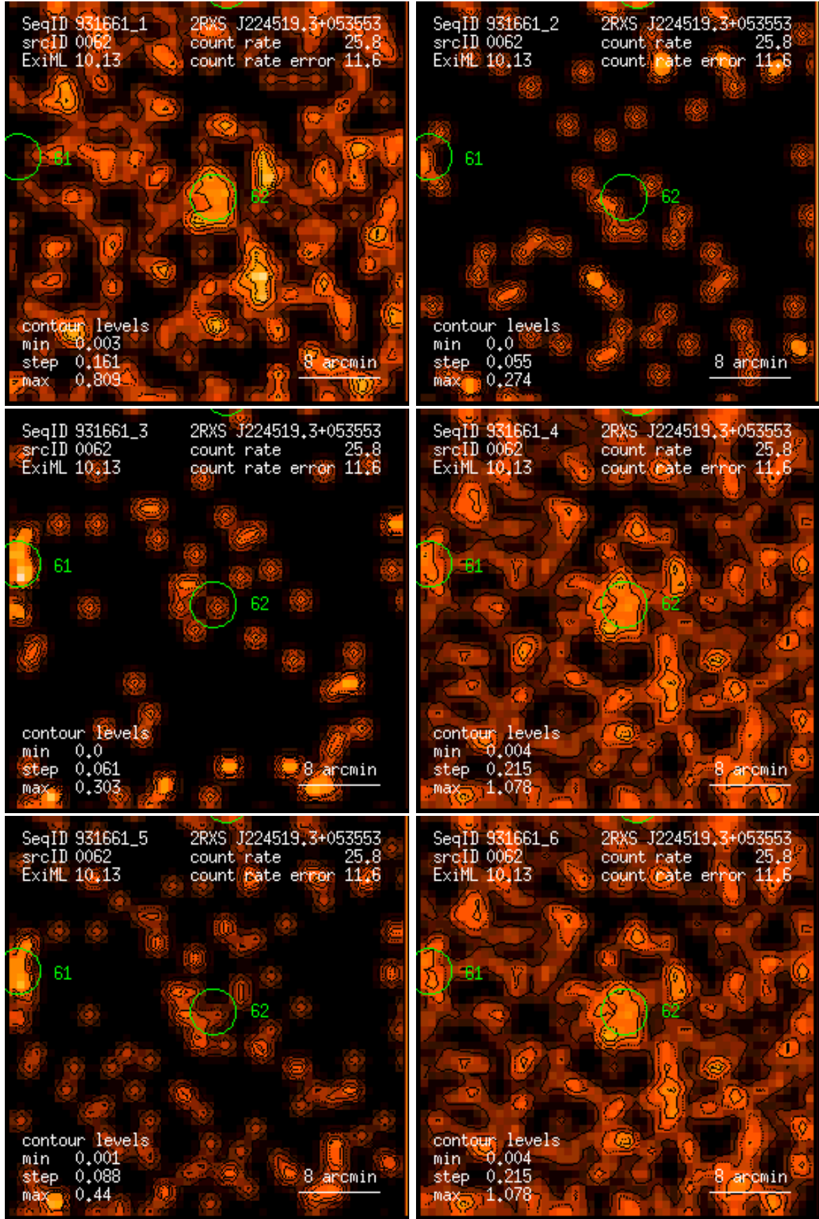
Figure 62: RASS 931661: detection 0062: band rate images, Gaussian filter: (1) PSPC channels 11 – 41, (2) 52 – 90, (3) 91 – 201, (4) 11 – 235, (5) 52 – 201, (6) 11 – 201. Broad band rates in counts/ks. Band rate contour levels in counts/ks/arcmin 2 .
