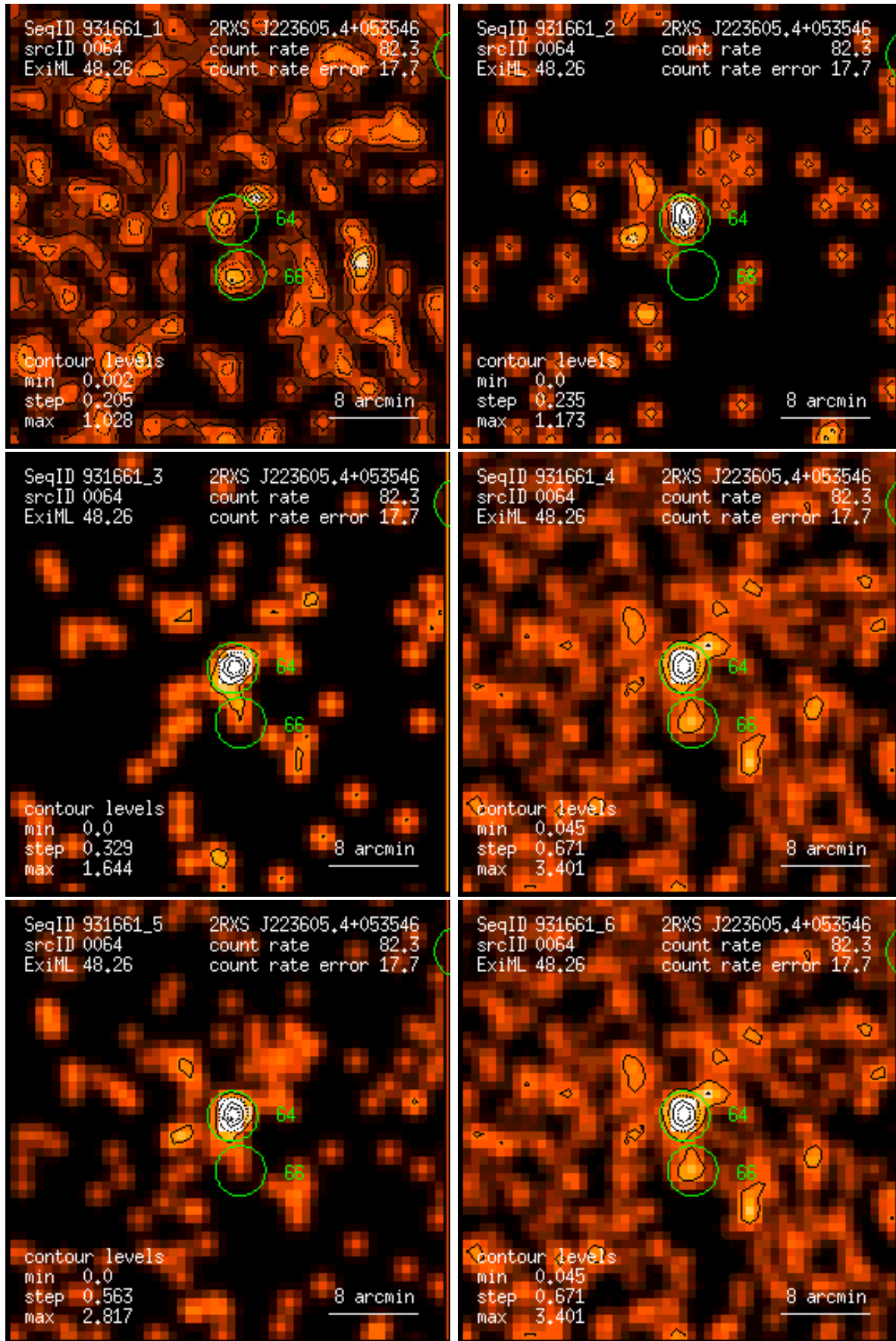
Figure 64: RASS 931661: detection 0064: band rate images, Gaussian filter: (1) PSPC channels 11 – 41, (2) 52 – 90, (3) 91 – 201, (4) 11 – 235, (5) 52 – 201, (6) 11 – 201. Broad band rates in counts/ks. Band rate contour levels in counts/ks/arcmin 2 .
