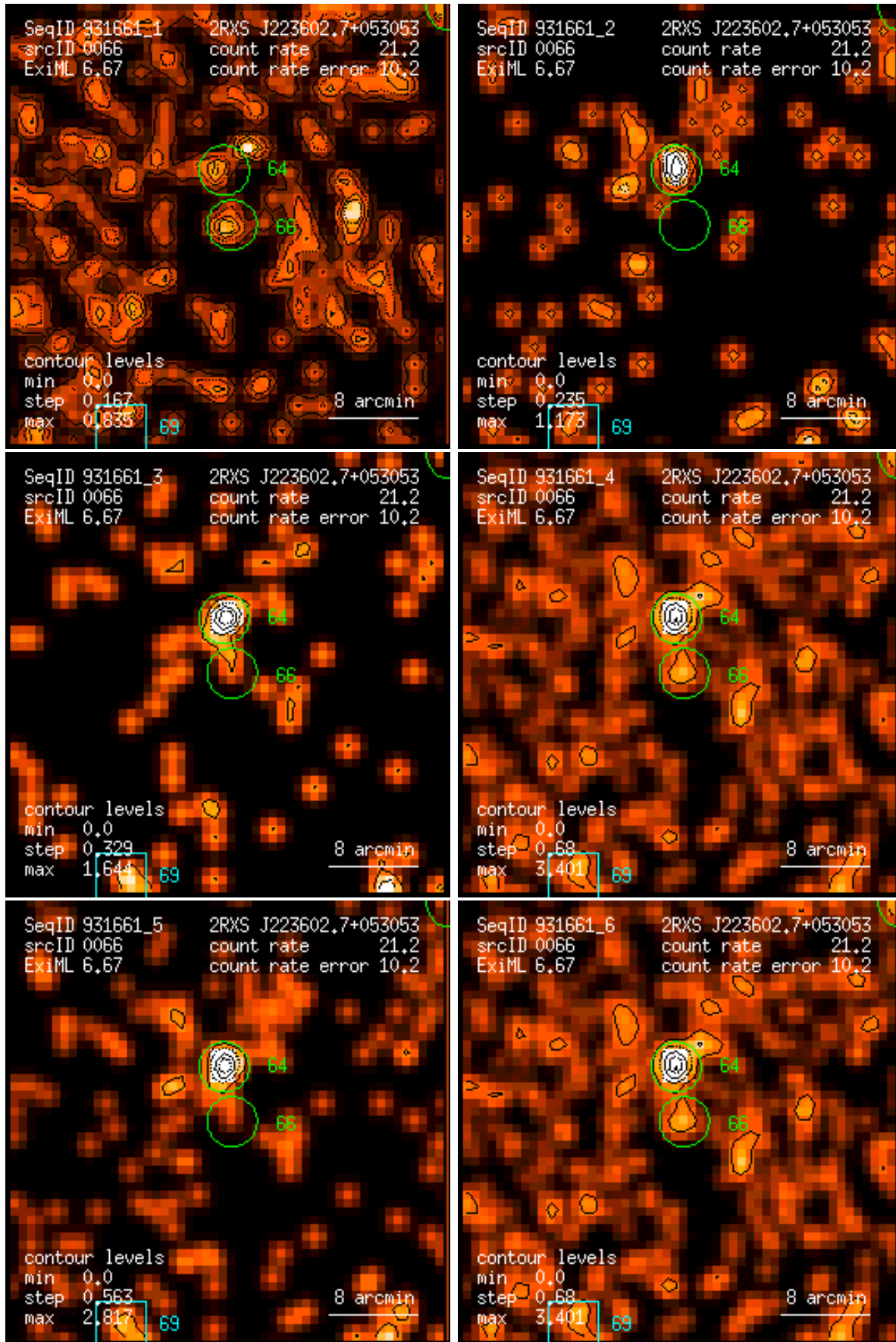
Figure 66: RASS 931661: detection 0066: band rate images, Gaussian filter: (1) PSPC channels 11 – 41, (2) 52 – 90, (3) 91 – 201, (4) 11 – 235, (5) 52 – 201, (6) 11 – 201. Broad band rates in counts/ks. Band rate contour levels in counts/ks/arcmin 2 .
