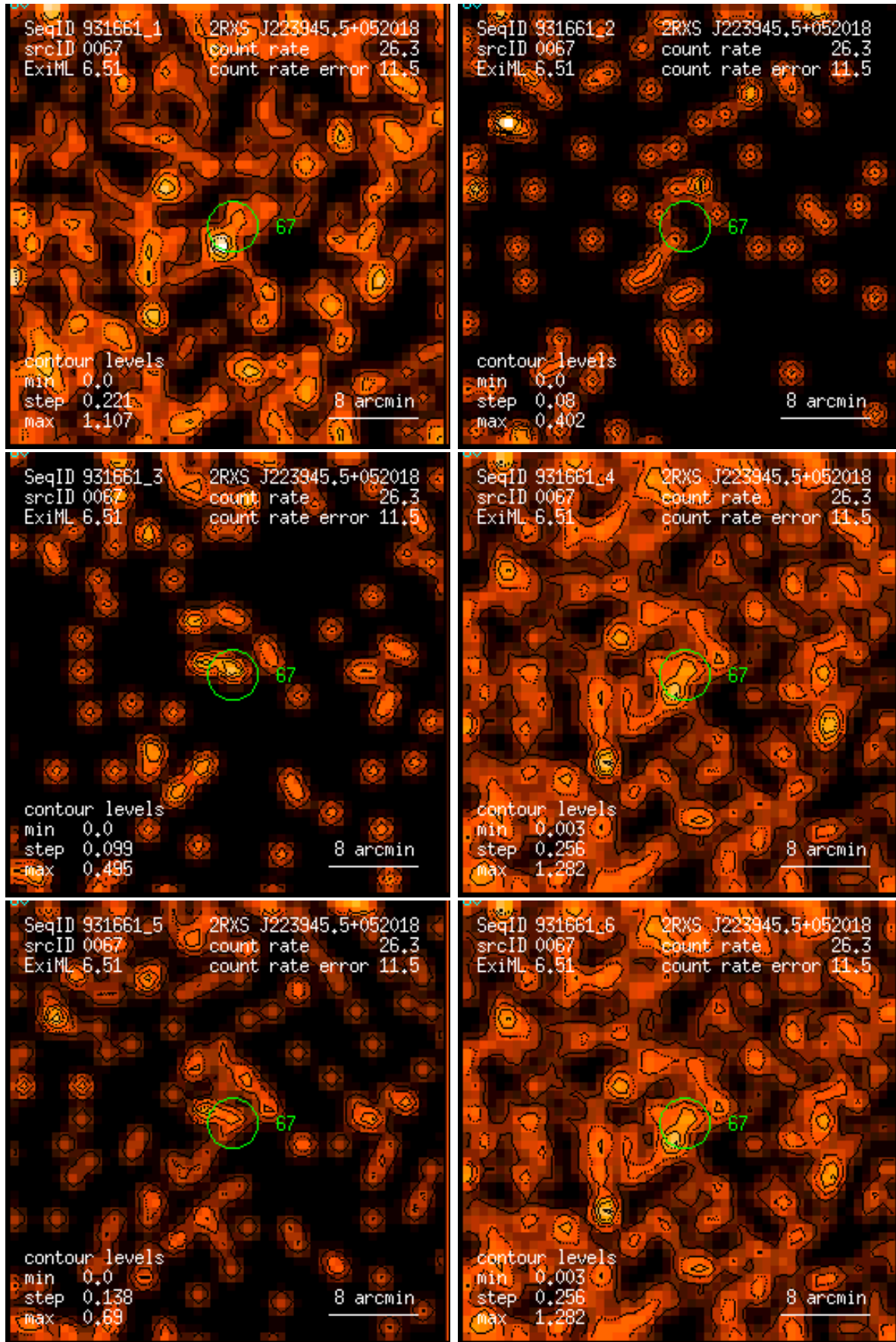
Figure 67: RASS 931661: detection 0067: band rate images, Gaussian filter: (1) PSPC channels 11 – 41, (2) 52 – 90, (3) 91 – 201, (4) 11 – 235, (5) 52 – 201, (6) 11 – 201. Broad band rates in counts/ks. Band rate contour levels in counts/ks/arcmin 2 .
